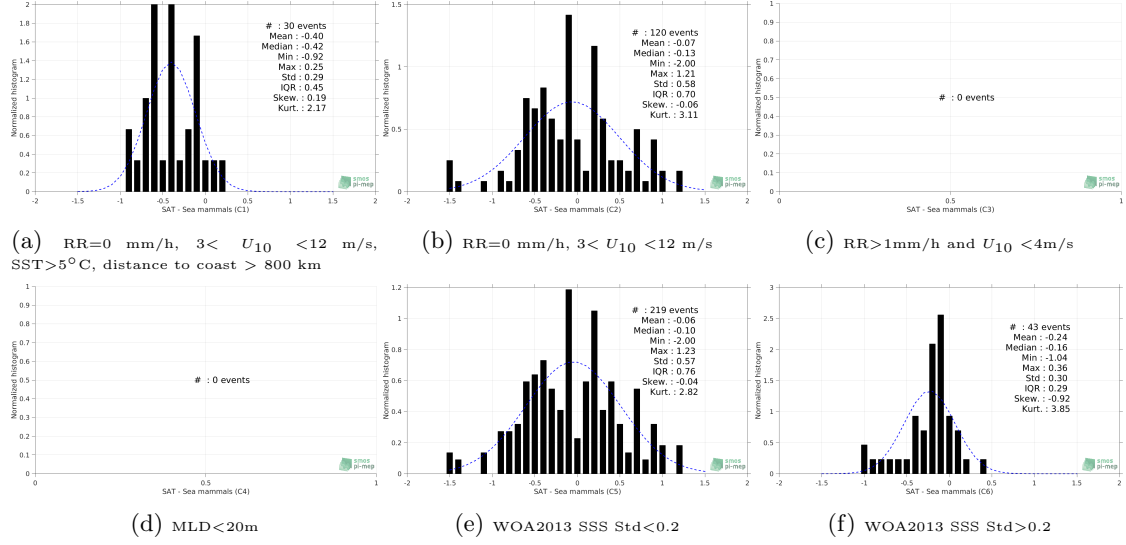
Figure 13: Normalized histogram of \Delta\text{SSS} (SMOS-L3-CATDS-IFREMER-CECOS-V2-MONTHLY-0.25DEG - Sea mammals) for 6 different subdatasets corresponding to: RR=0 mm/h, 3 < U_{10} < 12 m/s, SST > 5^\circ\text{C} , distance to coast > 800 km (a), RR=0 mm/h, 3 < U_{10} < 12 m/s (b), RR > 1 mm/h and U_{10} < 4 m/s (c), MLD < 20 m (d), WOA2013 SSS Std < 0.2 (e), WOA2013 SSS Std > 0.2 (f).
