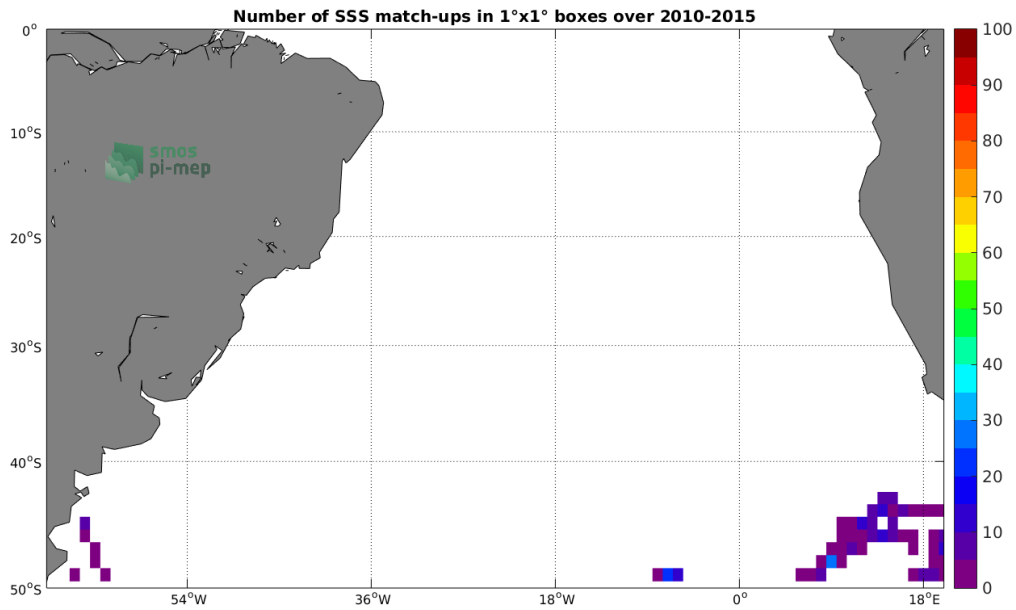
Figure 4: Number of SSS match-ups between Sea mammals SSS and the SMOS-L3-CATDS-IFREMER-CECOS-V2-MONTHLY-0.25DEG SSS product for the South Atlantic Ocean Pi-MEP region over 1^\circ \times 1^\circ boxes and for the full satellite product period.
