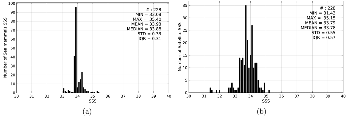
Figure 2: Histograms of SSS from Sea mammals (a) and SMOS-L3-CATDS-IFREMER-CECOS-V2-MONTHLY-0.25DEG (b) considering all match-up pairs per bins of 0.1 over the South Atlantic Ocean Pi-MEP region and for the full satellite product period.
