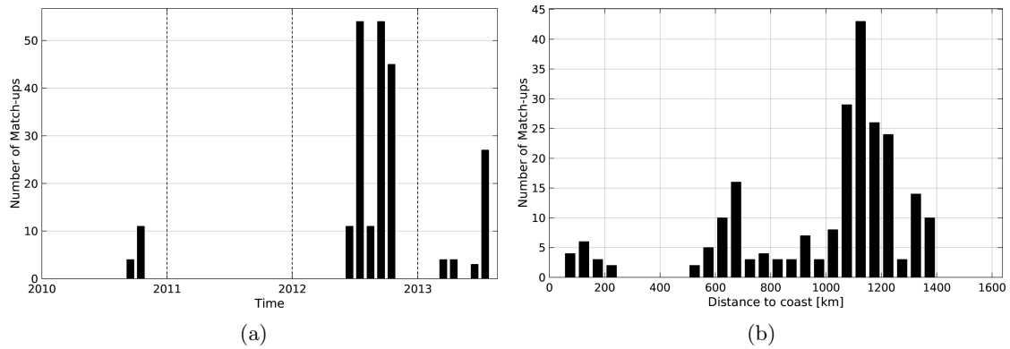
Figure 1: Number of match-ups between Sea mammals and SMOS-L3-CATDS-IFREMER-CECOS-V2-MONTHLY-0.25DEG SSS as a function of time (a) and as function of the distance to coast (b) over the South Atlantic Ocean Pi-MEP region and for the full satellite product period.
