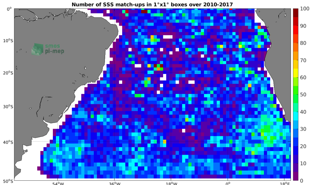
Figure 4: Number of SSS match-ups between Argo SSS and the SMOS SSS L3 v2 - Monthly - 0.25 Deg (CATDS-CECOS-IFREMER) SSS product for the South Atlantic Ocean Pi-MEP region over 1^\circ \times 1^\circ boxes and for the full satellite product period.
