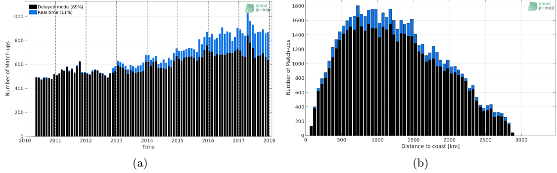
Figure 1: Number of match-ups between Argo and SMOS SSS L3 v2 - Monthly - 0.25 Deg (CATDS-CECOS-IFREMER) SSS as a function of time (a) and as function of the distance to coast (b) over the South Atlantic Ocean Pi-MEP region and for the full satellite product period.
