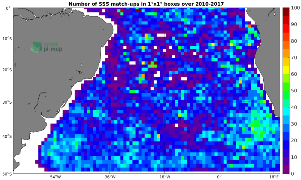
Figure 4: Number of SSS match-ups between Argos SSS and the SMOS SSS L3 v2 - Monthly - 0.25 Deg (CATDS-CECOS-IFREMER) SSS product for the South Atlantic Ocean Pi-MEP region over 1°x1° boxes and for the full satellite product period.
