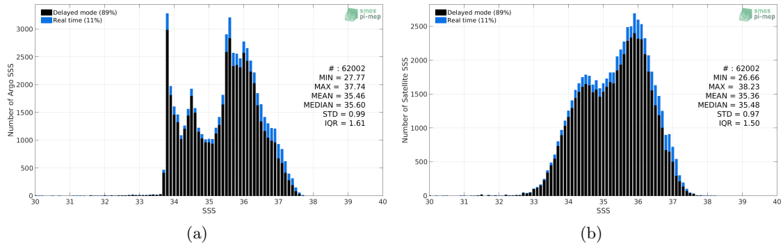
Figure 2: Histograms of SSS from Argo (a) and SMOS SSS L3 v2 - Monthly - 0.25 Deg (CATDS-CECOS-IFREMER) (b) considering all match-up pairs per bins of 0.1 over the South Atlantic Ocean Pi-MEP region and for the full satellite product period.
