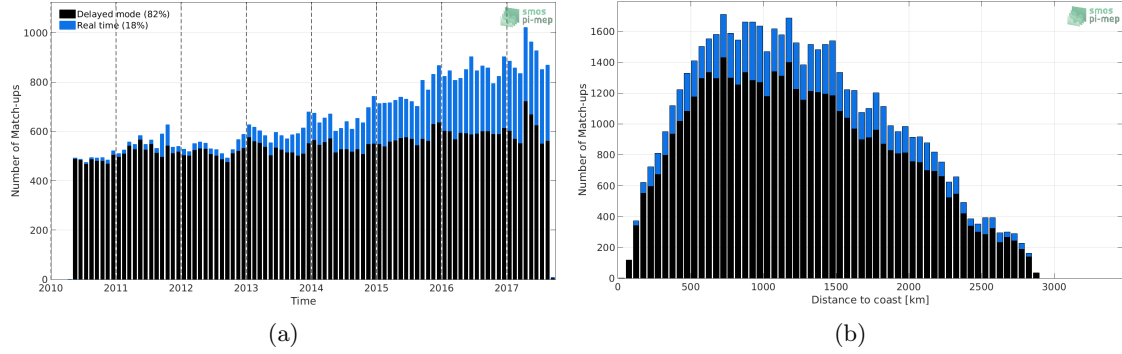
Figure 1: Number of match-ups between Argo and SMOS L3 v2 - Monthly - 0.25 Deg (CATDS-CECOS-IFREMER) SSS as a function of time (a) and as function of the distance to coast (b) over the South Atlantic Ocean Pi-MEP region and for the full satellite product period.
