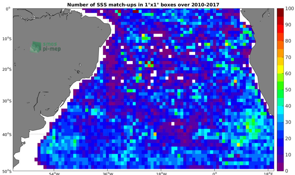
Figure 4: Number of SSS match-ups between Argo SSS and the SMOS L3 v2 - Monthly - 0.25 Deg (CATDS-CECOS-IFREMER) SSS product for the South Atlantic Ocean Pi-MEP region over 1^\circ \times 1^\circ boxes and for the full satellite product period.
