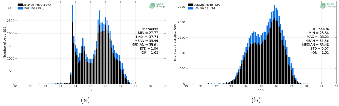
Figure 2: Histograms of SSS from Argo (a) and SMOS L3 v2 - Monthly - 0.25 Deg (CATDS-CECOS-IFREMER) (b) considering all match-up pairs per bins of 0.1 over the South Atlantic Ocean Pi-MEP region and for the full satellite product period.
