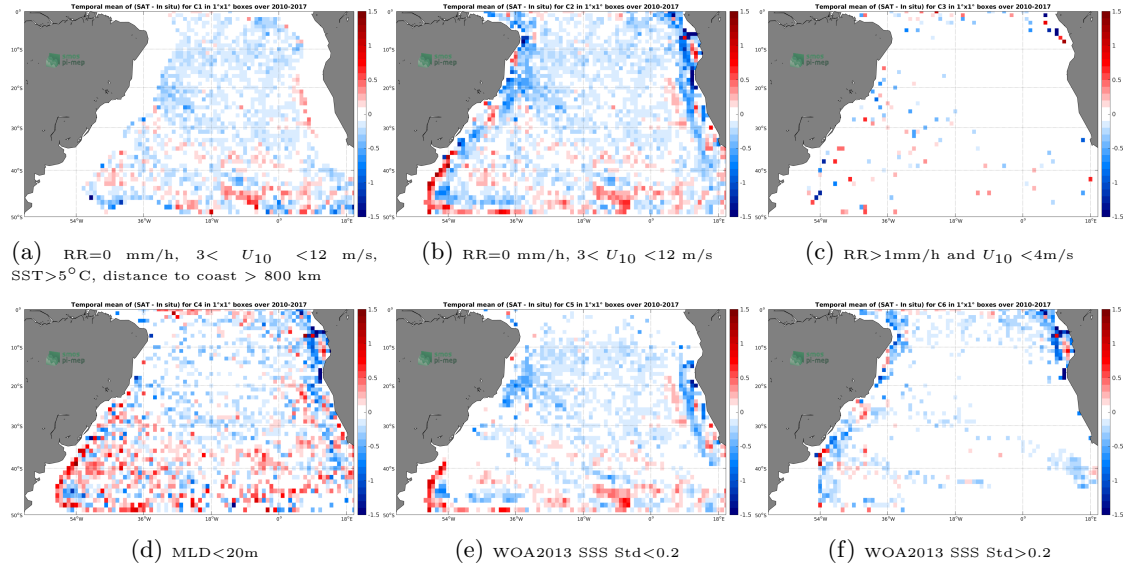
Figure 12: Temporal mean gridded over spatial boxes of size 1^\circ \times 1^\circ of \Delta SSS (SMOS L3 v2 - Monthly - 0.25^\circ Deg (CATDS-CECOS-IFREMER) - Argo) for 6 different subdatasets corresponding to: RR=0 mm/h, 3 < U_{10} < 12 m/s, SST > 5^\circ\text{C} , distance to coast > 800 km (a), RR=0 mm/h, 3 < U_{10} < 12 m/s (b), RR > 1 mm/h and U_{10} < 4 m/s (c), MLD < 20 m (d), WOA2013 SSS Std < 0.2 (e), WOA2013 SSS Std > 0.2 (f).
