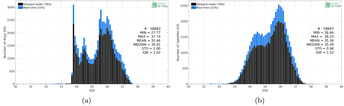
Figure 2: Histograms of SSS from Argo (a) and SMOS-L3-CATDS-IFREMER-CECOS-V2-MONTHLY-0.25DEG (b) considering all match-up pairs per bins of 0.1 over the South Atlantic Ocean Pi-MEP region and for the full satellite product period.
