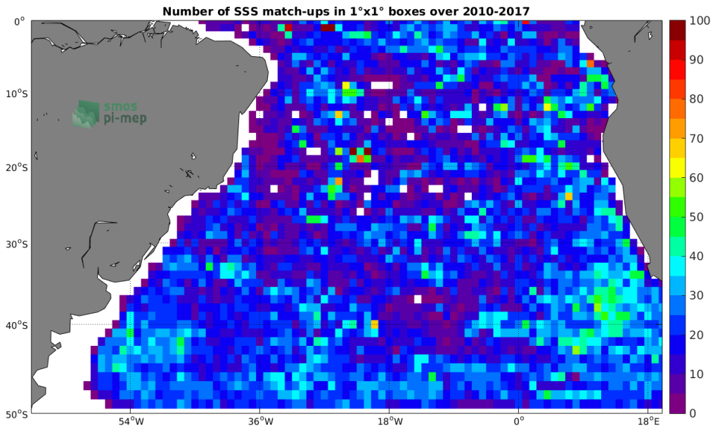
Figure 4: Number of SSS match-ups between Argo SSS and the SMOS-L3-CATDS-IFREMER-CECOS-V2-MONTHLY-0.25DEG SSS product for the South Atlantic Ocean Pi-MEP region over 1°x1° boxes and for the full satellite product period.
