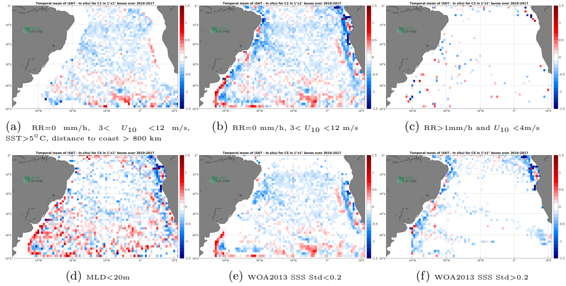
Figure 12: Temporal mean gridded over spatial boxes of size 1^\circ \times 1^\circ of \Delta SSS (SMOS-L3-CATDS-IFREMER-CECOS-V2-MONTHLY-0.25DEG - Argo) for 6 different subdatasets corresponding to: RR=0 mm/h, 3 < U_{10} < 12 m/s, SST > 5^\circ\text{C} , distance to coast > 800 km (a), RR=0 mm/h, 3 < U_{10} < 12 m/s (b), RR > 1 mm/h and U_{10} < 4 m/s (c), MLD < 20 m (d), WOA2013 SSS Std < 0.2 (e), WOA2013 SSS Std > 0.2 (f).
