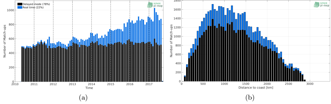
Figure 1: Number of match-ups between Argo and SMOS-L3-CATDS-IFREMER-CECOS-V2-MONTHLY-0.25DEG SSS as a function of time (a) and as function of the distance to coast (b) over the South Atlantic Ocean Pi-MEP region and for the full satellite product period.
