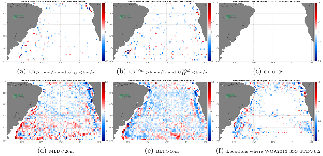
Figure 12: Temporal mean gridded over spatial boxes of size 1^\circ \times 1^\circ of \Delta\text{SSS} (SMOS-L3-CATDS-IFREMER-CECOS-V2-MONTHLY-0.25DEG - Argo) for 6 different subdatasets corresponding to: RR > 1\text{mm/h} and U_{10} < 5\text{m/s} (a), RR^{10d} > 5\text{mm/h} and U_{10}^{10d} < 5\text{m/s} (b), C1 U C2 (c), MLD < 20\text{m} (d), BLT > 10\text{m} (e), Locations where WOA2013 SSS STD > 0.2 (f).
