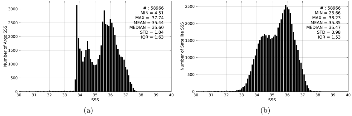
Figure 2: Histograms of SSS from Argo (a) and SMOS-L3-CATDS-IFREMER-CECOS-V2-MONTHLY-0.25DEG (b) considering all match-up pairs per bins of 0.1 over the South Atlantic Ocean Pi-MEP region and for the full satellite product period.
