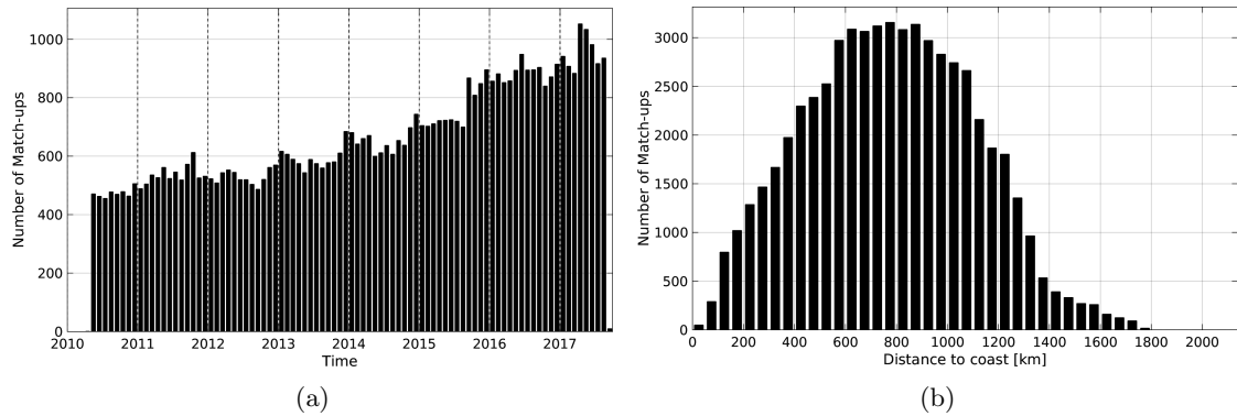
Figure 1: Number of match-ups between Argo and SMOS-L3-CATDS-IFREMER-CECOS-V2-MONTHLY-0.25DEG SSS as a function of time (a) and as function of the distance to coast (b) over the South Atlantic Ocean Pi-MEP region and for the full satellite product period.
