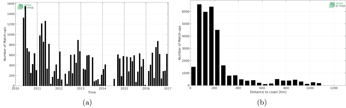
Figure 1: Number of match-ups between TSG-LEGOS-DM and SMOS-L3-CATDS-CECOS-IFREMER-V2-1DAY-0.5DEG SSS as a function of time (a) and as function of the distance to coast (b) over the South Atlantic Ocean Pi-MEP region and for the full satellite product period.
