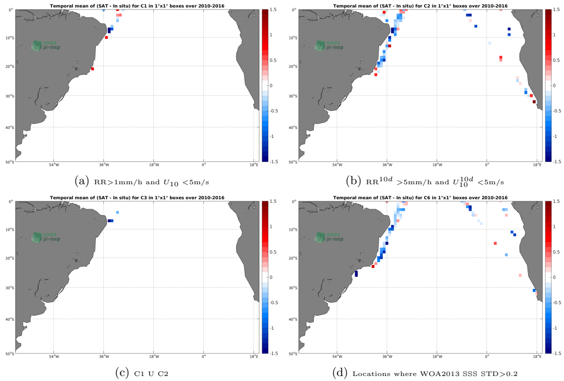
Figure 12: Temporal mean gridded over spatial boxes of size 1^\circ \times 1^\circ of \Delta SSS (SMOS-L3-CATDS-CECOS-IFREMER-V2-1DAY-0.5DEG - TSG-LEGOS-DM) for 4 different subdatasets corresponding to: RR > 1mm/h and U_{10} < 5\text{m/s} (a), RR^{10d} > 5\text{mm/h} and U_{10}^{10d} < 5\text{m/s} (b), C1 U C2 (c), Locations where WOA2013 SSS STD > 0.2 (d).
