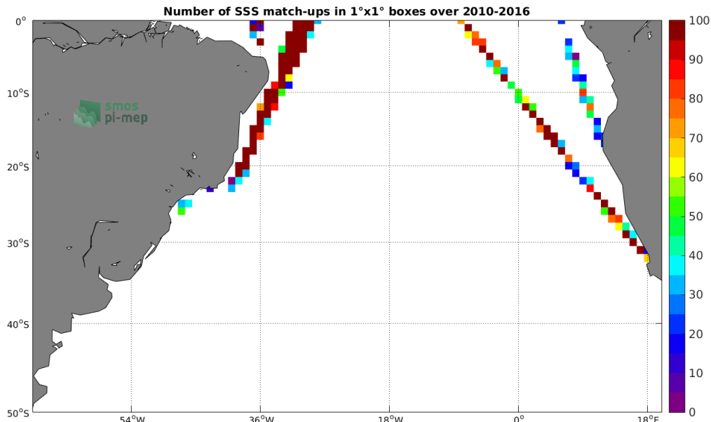
Figure 4: Number of SSS match-ups between TSG-LEGOS-DM SSS and the SMOS-L3-CATDS-CECOS-IFREMER-V2-1DAY-0.5DEG SSS product for the South Atlantic Ocean Pi-MEP region over 1°x1° boxes and for the full satellite product period.
