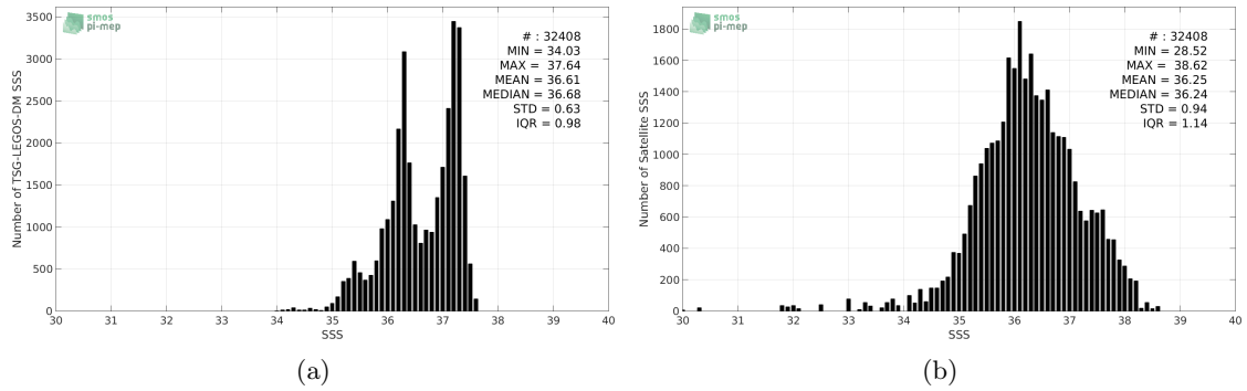
Figure 2: Histograms of SSS from TSG-LEGOS-DM (a) and SMOS-L3-CATDS-CECOS-IFREMER-V2-1DAY-0.5DEG (b) considering all match-up pairs per bins of 0.1 over the South Atlantic Ocean Pi-MEP region and for the full satellite product period.
