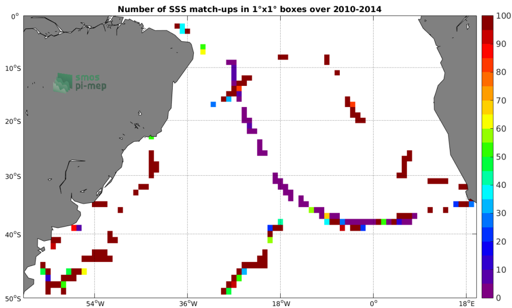
Figure 4: Number of SSS match-ups between TSG-GOSUD-Sailing-ship SSS and the SMOS-L3-CATDS-CECOS-IFREMER-V2-1DAY-0.5DEG SSS product for the South Atlantic Ocean Pi-MEP region over 1^\circ \times 1^\circ boxes and for the full satellite product period.
