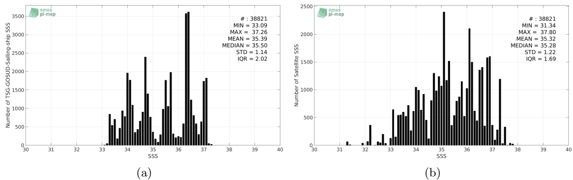
Figure 2: Histograms of SSS from TSG-GOSUD-Sailing-ship (a) and SMOS-L3-CATDS-CECOS-IFREMER-V2-1DAY-0.5DEG (b) considering all match-up pairs per bins of 0.1 over the South Atlantic Ocean Pi-MEP region and for the full satellite product period.
