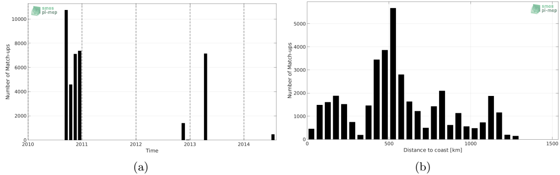
Figure 1: Number of match-ups between TSG-GOSUD-Sailing-ship and SMOS-L3-CATDS-CECOS-IFREMER-V2-1DAY-0.5DEG SSS as a function of time (a) and as function of the distance to coast (b) over the South Atlantic Ocean Pi-MEP region and for the full satellite product period.
