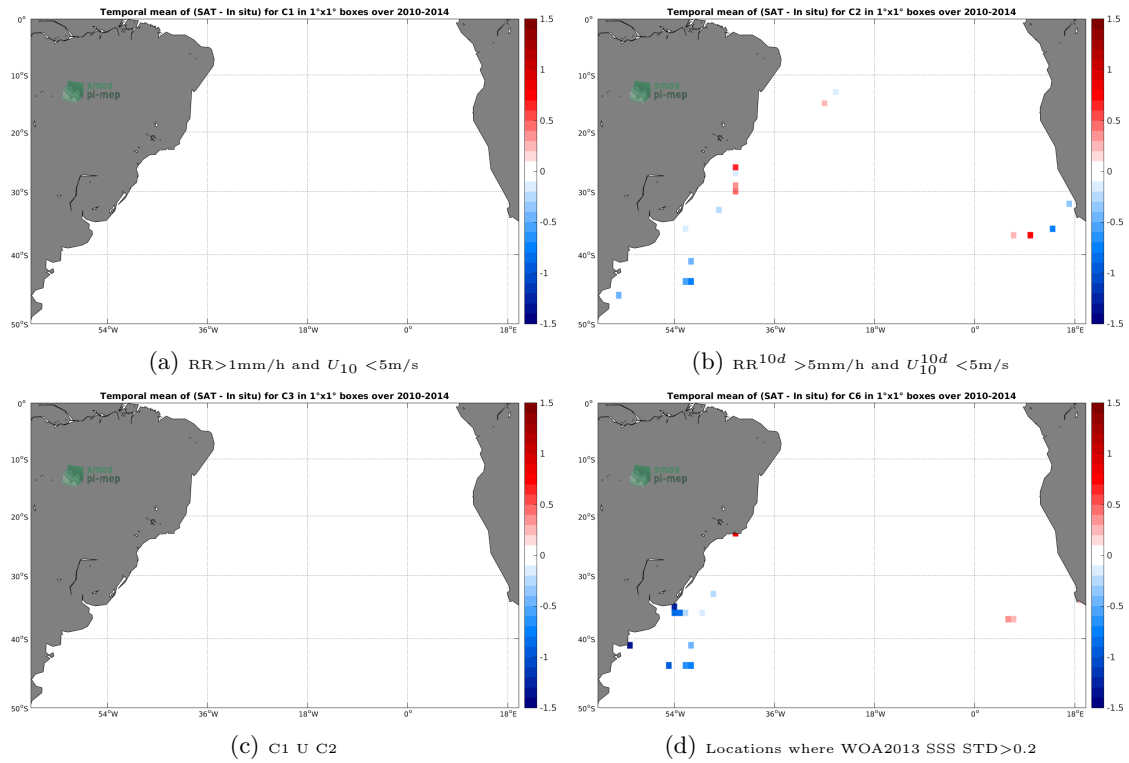
Figure 12: Temporal mean gridded over spatial boxes of size 1^\circ \times 1^\circ of \Delta SSS (SMOS-L3-CATDS-CECOS-IFREMER-V2-1DAY-0.5DEG - TSG-GOSUD-Sailing-ship) for 4 different subdatasets corresponding to:RR > 1 mm/h and U_{10} < 5 m/s (a), RR^{10d} > 5 mm/h and U_{10}^{10d} < 5 m/s (b), C1 U C2 (c),Locations where WOA2013 SSS STD > 0.2 (d).
