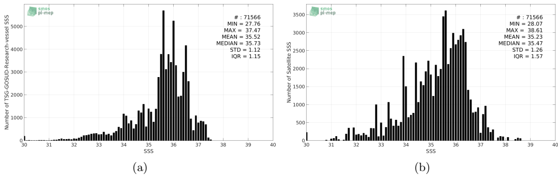
Figure 2: Histograms of SSS from TSG-GOSUD-Research-vessel (a) and SMOS-L3-CATDS-CECOS-IFREMER-V2-1DAY-0.5DEG (b) considering all match-up pairs per bins of 0.1 over the South Atlantic Ocean Pi-MEP region and for the full satellite product period.
