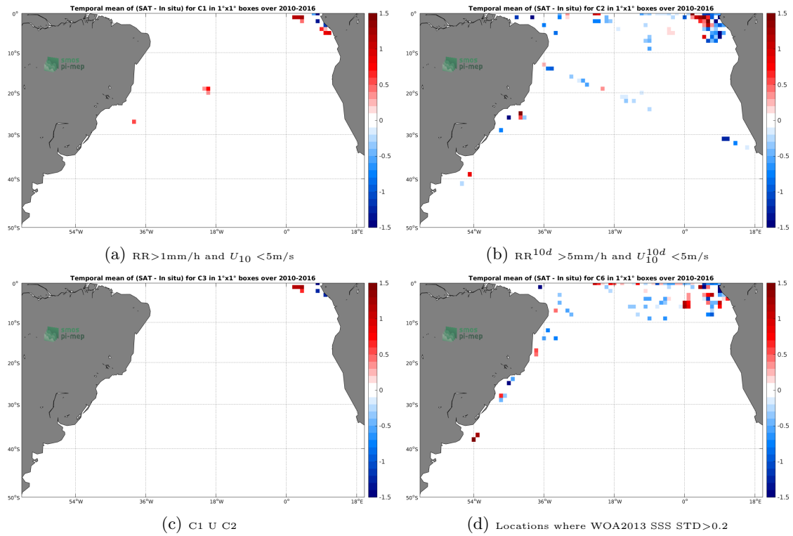
Figure 12: Temporal mean gridded over spatial boxes of size 1^\circ \times 1^\circ of \Delta SSS (SMOS-L3-CATDS-CECOS-IFREMER-V2-1DAY-0.5DEG - TSG-GOSUD-Research-vessel) for 4 different subdatasets corresponding to: RR > 1mm/h and U_{10} < 5\text{m/s} (a), RR^{10d} > 5\text{mm/h} and U_{10}^{10d} < 5\text{m/s} (b), C1 U C2 (c), Locations where WOA2013 SSS STD > 0.2 (d).
