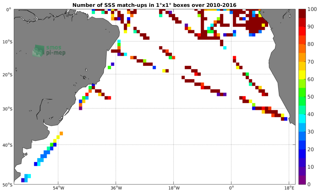
Figure 4: Number of SSS match-ups between TSG-GOSUD-Research-vessel SSS and the SMOS-L3-CATDS-CECOS-IFREMER-V2-1DAY-0.5DEG SSS product for the South Atlantic Ocean Pi-MEP region over 1°x1° boxes and for the full satellite product period.
