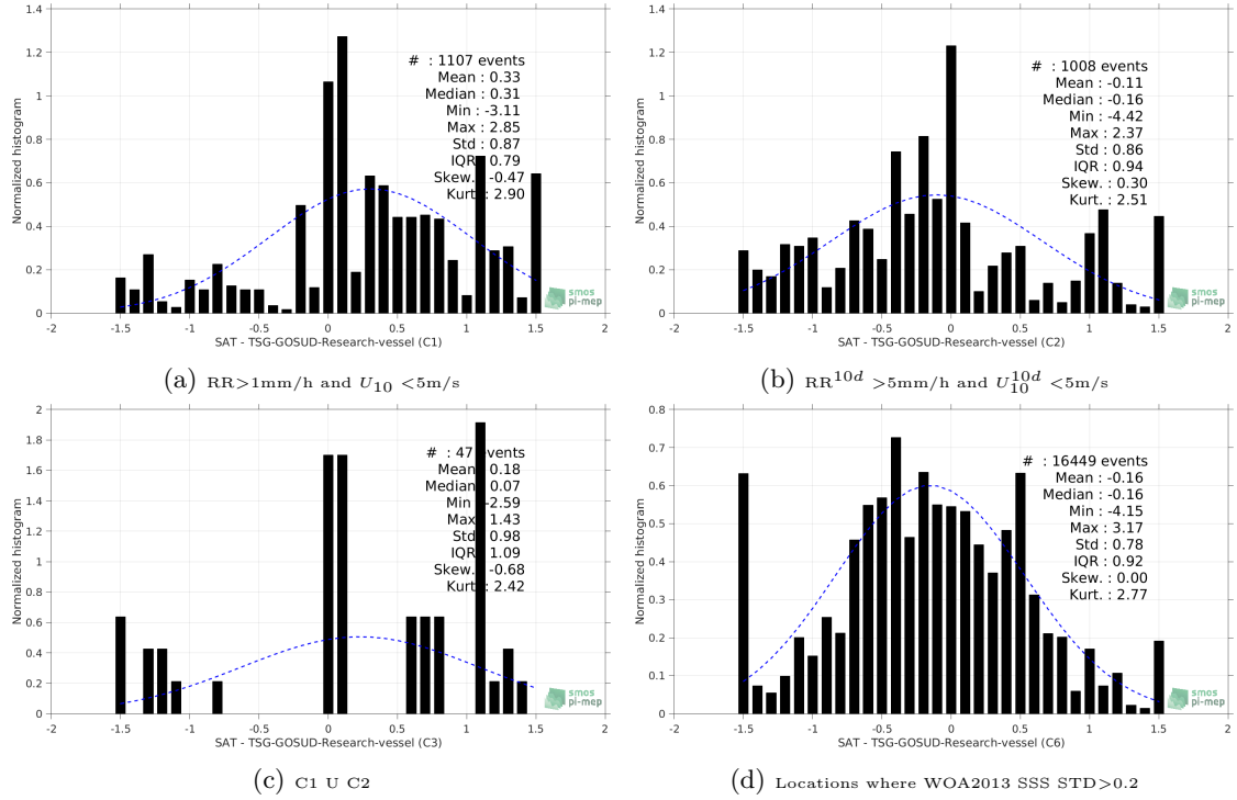
Figure 13: Normalized histogram of \Delta SSS (SMOS-L3-CATDS-CECOS-IFREMER-V2-1DAY-0.5DEG - TSG-GOSUD-Research-vessel) for 6 different subdatasets corresponding to: RR > 1mm/h and U_{10} < 5 m/s (a), RR^{10d} > 5 mm/h and U_{10}^{10d} < 5 m/s (b), C1 U C2 (c), Locations where WOA2013 SSS STD > 0.2 (d).
