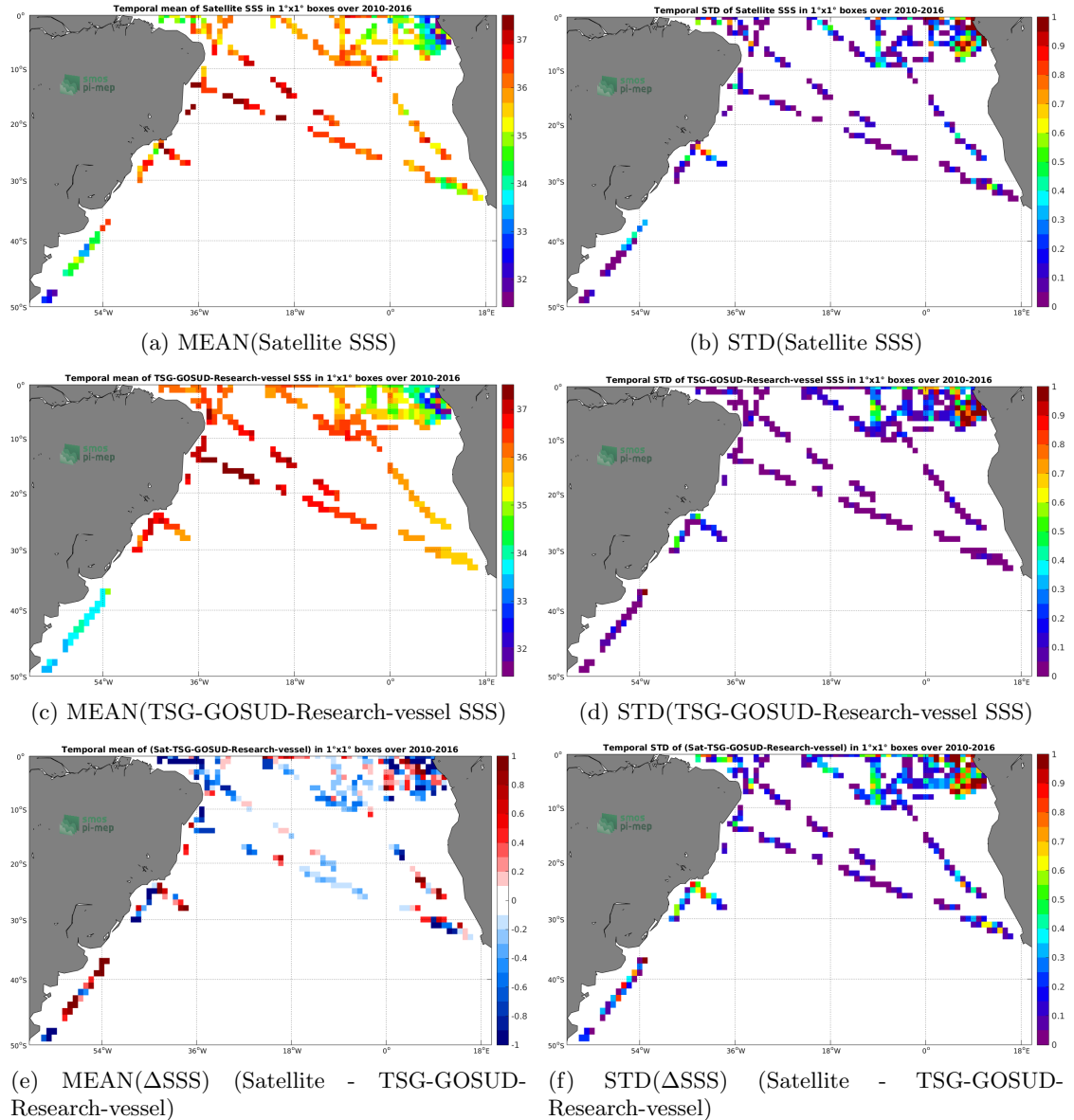
Figure 6: Temporal mean (left) and STD (right) of SSS from SMOS-L3-CATDS-CECOS-IFREMER-V2-1DAY-0.5DEG (top), TSG-GOSUD-Research-vessel (middle), and of \Delta SSS (Satellite - TSG-GOSUD-Research-vessel). Only match-up pairs are used to generate these maps.
