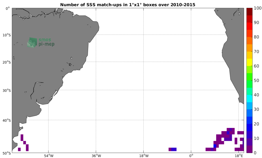
Figure 4: Number of SSS match-ups between Sea mammals SSS and the SMOS-L3-CATDS-CECOS-IFREMER-V2-1DAY-0.5DEG SSS product for the South Atlantic Ocean Pi-MEP region over 1^\circ \times 1^\circ boxes and for the full satellite product period.
