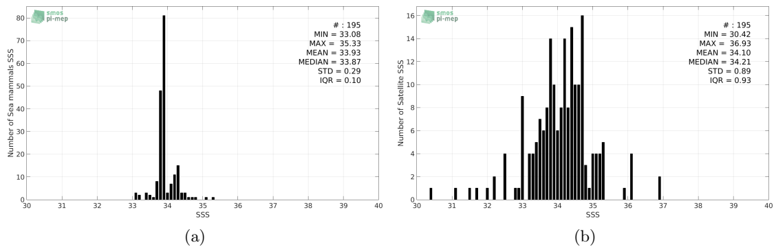
Figure 2: Histograms of SSS from Sea mammals (a) and SMOS-L3-CATDS-CECOS-IFREMER-V2-1DAY-0.5DEG (b) considering all match-up pairs per bins of 0.1 over the South Atlantic Ocean Pi-MEP region and for the full satellite product period.
