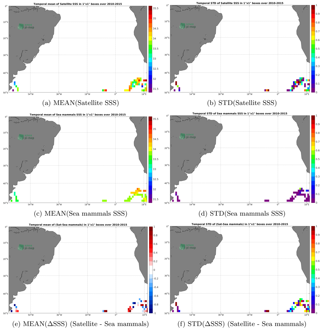
Figure 6: Temporal mean (left) and STD (right) of SSS from SMOS-L3-CATDS-CECOS-IFREMER-V2-1DAY-0.5DEG (top), Sea mammals (middle), and of \Delta SSS (Satellite - Sea mammals). Only match-up pairs are used to generate these maps.
