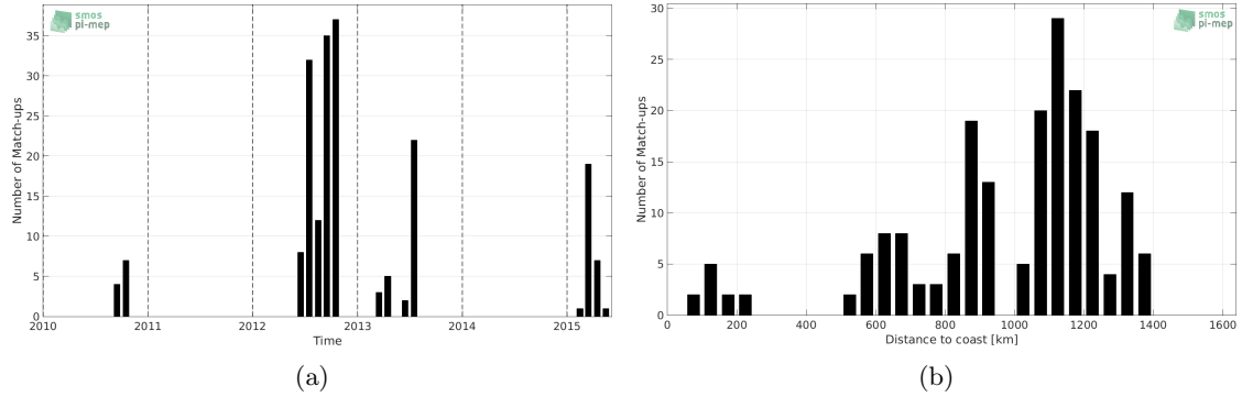
Figure 1: Number of match-ups between Sea mammals and SMOS-L3-CATDS-CECOS-IFREMER-V2-1DAY-0.5DEG SSS as a function of time (a) and as function of the distance to coast (b) over the South Atlantic Ocean Pi-MEP region and for the full satellite product period.
