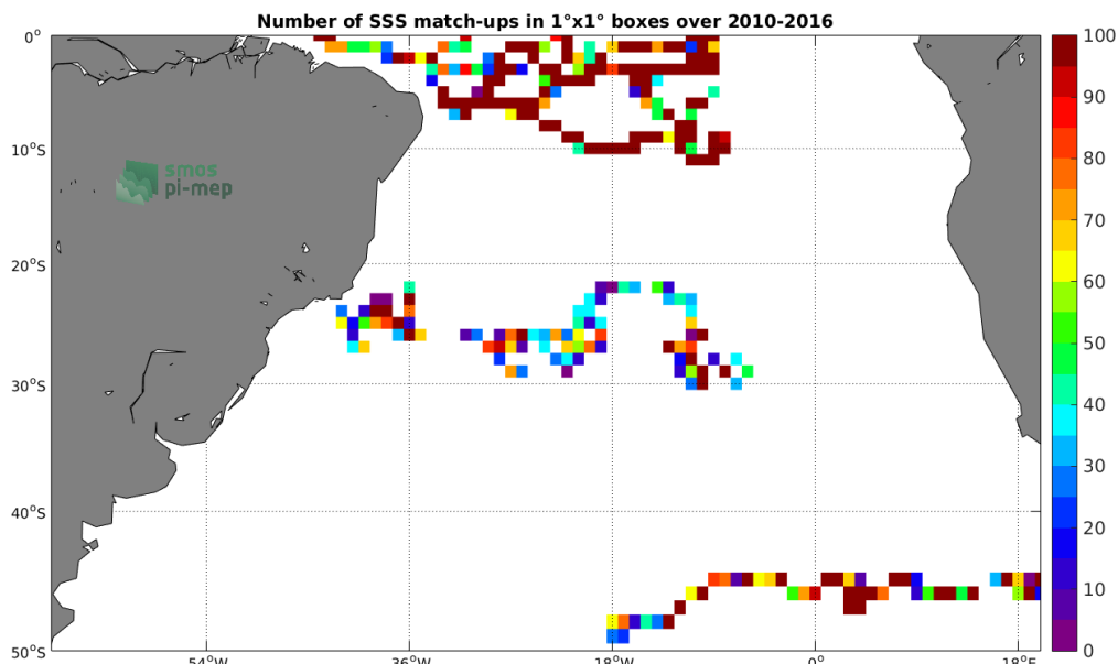
Figure 3: Number of SSS match-ups between Surface drifters SSS and the SMOS-L3-CATDS-CECOS-IFREMER-V2-1DAY-0.5DEG SSS product for the South Atlantic Ocean Pi-MEP region over 1°x1° boxes and for the full satellite product period.
