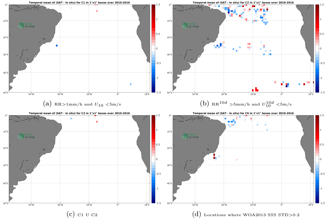
Figure 11: Temporal mean gridded over spatial boxes of size 1^\circ \times 1^\circ of \Delta SSS (SMOS-L3-CATDS-CECOS-IFREMER-V2-1DAY-0.5DEG - Surface drifters) for 4 different subdatasets corresponding to: RR > 1mm/h and U_{10} < 5\text{m/s} (a), RR^{10d} > 5\text{mm/h} and U_{10}^{10d} < 5\text{m/s} (b), C1 U C2 (c), Locations where WOA2013 SSS STD > 0.2 (d).
