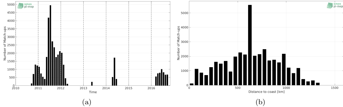
Figure 1: Number of match-ups between Surface drifters and SMOS-L3-CATDS-CECOS-IFREMER-V2-1DAY-0.5DEG SSS as a function of time (a) and as function of the distance to coast (b) over the South Atlantic Ocean Pi-MEP region and for the full satellite product period.
