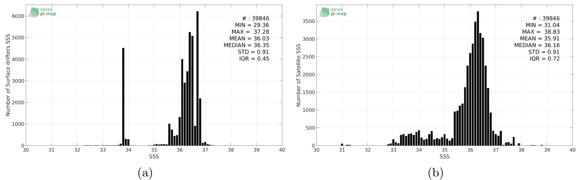
Figure 2: Histograms of SSS from Surface drifters (a) and SMOS-L3-CATDS-CECOS-IFREMER-V2-1DAY-0.5DEG (b) considering all match-up pairs per bins of 0.1 over the South Atlantic Ocean Pi-MEP region and for the full satellite product period.
