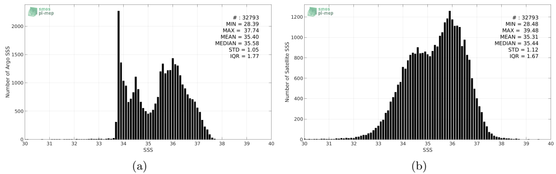
Figure 2: Histograms of SSS from Argo (a) and SMOS-L3-CATDS-CECOS-IFREMER-V2-1DAY-0.5DEG (b) considering all match-up pairs per bins of 0.1 over the South Atlantic Ocean Pi-MEP region and for the full satellite product period.
