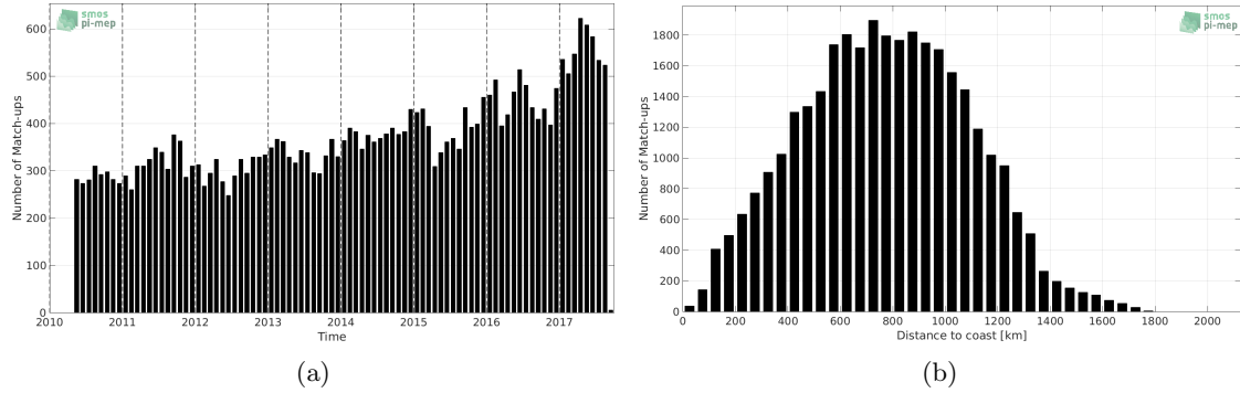
Figure 1: Number of match-ups between Argo and SMOS-L3-CATDS-CECOS-IFREMER-V2-1DAY-0.5DEG SSS as a function of time (a) and as function of the distance to coast (b) over the South Atlantic Ocean Pi-MEP region and for the full satellite product period.
