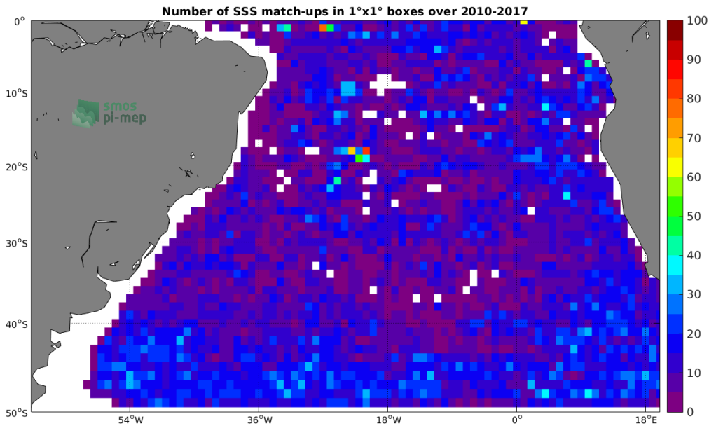
Figure 4: Number of SSS match-ups between Argo SSS and the SMOS-L3-CATDS-CECOS-IFREMER-V2-1DAY-0.5DEG SSS product for the South Atlantic Ocean Pi-MEP region over 1^\circ \times 1^\circ boxes and for the full satellite product period.
