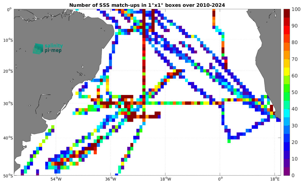
Figure 5: Number of SSS match-ups between TSG (SAMOS) SSS and the SMOS SSS L3 v335 - Monthly - 25 km (CATDS-CPDC) SSS product for the South Atlantic Ocean Pi-MEP region over 1^\circ \times 1^\circ boxes and for the full satellite product period.
