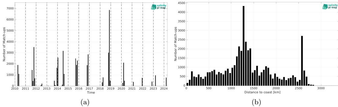
Figure 2: Number of match-ups between TSG (SAMOS) and SMOS SSS L3 v335 - Monthly - 25 km (CATDS-CPDC) SSS as a function of time (a) and as function of the distance to coast (b) over the South Atlantic Ocean Pi-MEP region and for the full satellite product period.
