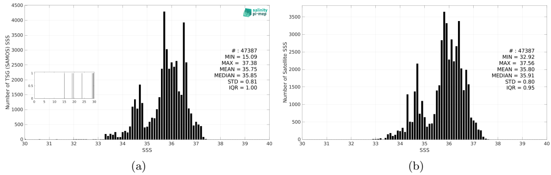
Figure 3: Histograms of SSS from TSG (SAMOS) (a) and SMOS SSS L3 v335 - Monthly - 25 km (CATDS-CPDC) (b) considering all match-up pairs per bins of 0.1 over the South Atlantic Ocean Pi-MEP region and for the full satellite product period.
