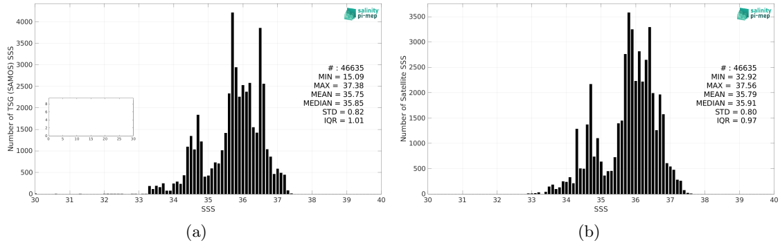
Figure 2: Histograms of SSS from TSG (SAMOS) (a) and SMOS SSS L3 v335 - Monthly - 25 km (CATDS-CPDC) (b) considering all match-up pairs per bins of 0.1 over the South Atlantic Ocean Pi-MEP region and for the full satellite product period.
