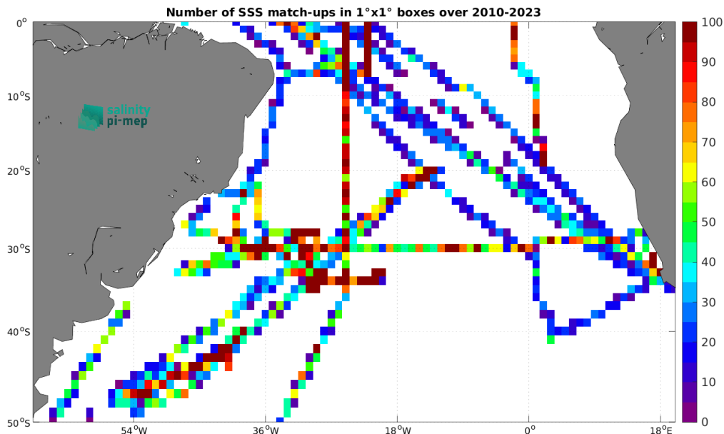
Figure 4: Number of SSS match-ups between TSG (SAMOS) SSS and the SMOS SSS L3 v335 - Monthly - 25 km (CATDS-CPDC) SSS product for the South Atlantic Ocean Pi-MEP region over 1^\circ \times 1^\circ boxes and for the full satellite product period.
