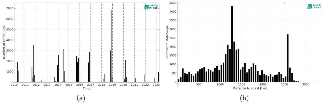
Figure 1: Number of match-ups between TSG (SAMOS) and SMOS SSS L3 v335 - Monthly - 25 km (CATDS-CPDC) SSS as a function of time (a) and as function of the distance to coast (b) over the South Atlantic Ocean Pi-MEP region and for the full satellite product period.
