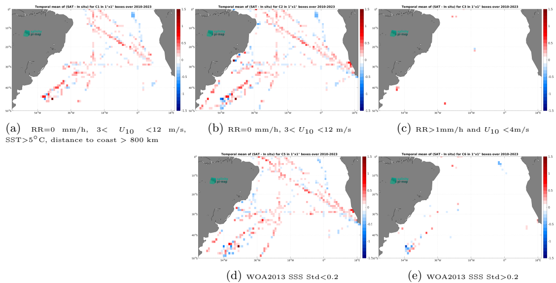
Figure 12: Temporal mean gridded over spatial boxes of size 1^\circ \times 1^\circ of \Delta\text{SSS} (SMOS SSS L3 v335 - Monthly - 25 km (CATDS-CPDC) - TSG (SAMOS)) for 5 different subdatasets corresponding to:RR=0 mm/h, 3 < U_{10} < 12 m/s, SST >5^\circ\text{C} , distance to coast > 800 km (a), RR=0 mm/h, 3 < U_{10} < 12 m/s (b), RR >1 mm/h and U_{10} < 4 m/s (c), WOA2013 SSS Std <0.2 (d), WOA2013 SSS Std >0.2 (e).
