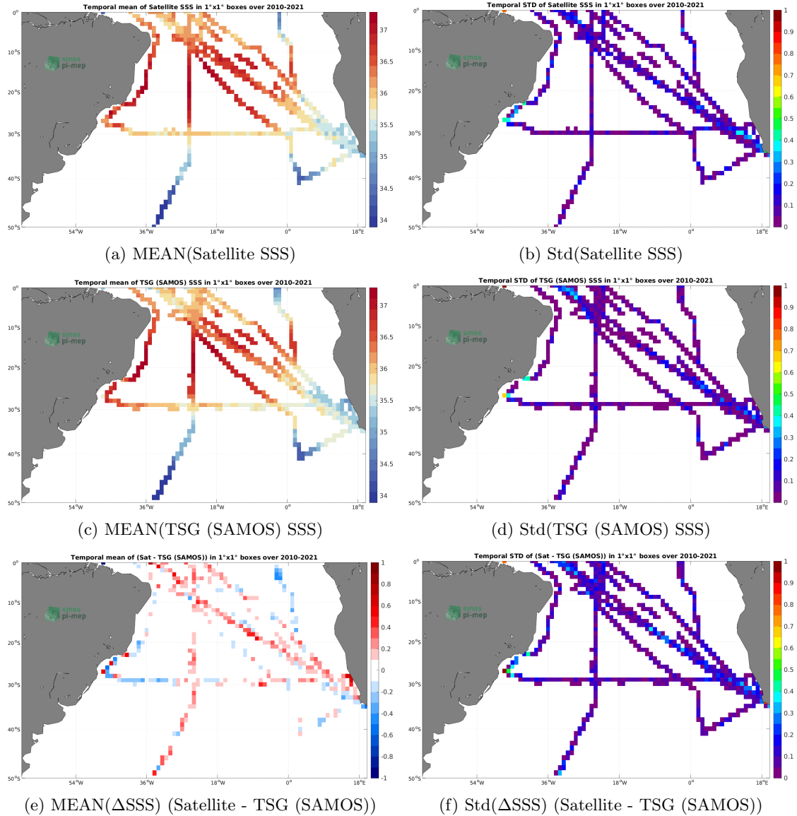
Figure 6: Temporal mean (left) and Std (right) of SSS from SMOS SSS L3 v335 - Monthly - 25 km (CATDS-CPDC) (top), TSG (SAMOS) (middle), and of \Delta SSS (Satellite - TSG (SAMOS)). Only match-up pairs are used to generate these maps.
