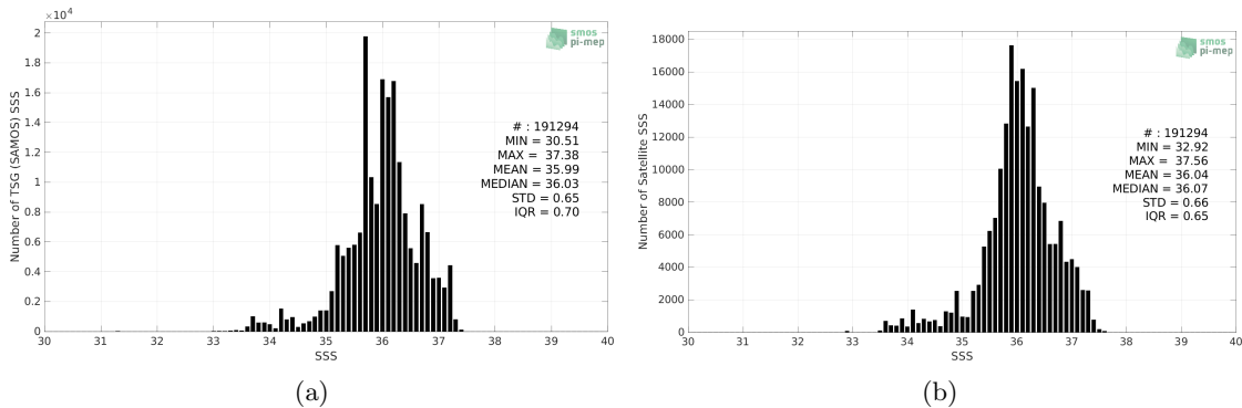
Figure 2: Histograms of SSS from TSG (SAMOS) (a) and SMOS SSS L3 v335 - Monthly - 25 km (CATDS-CPDC) (b) considering all match-up pairs per bins of 0.1 over the South Atlantic Ocean Pi-MEP region and for the full satellite product period.
