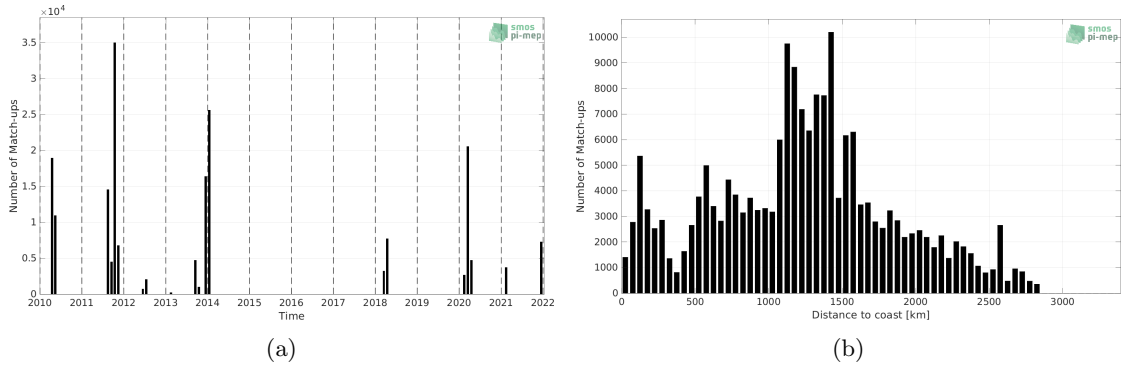
Figure 1: Number of match-ups between TSG (SAMOS) and SMOS SSS L3 v335 - Monthly - 25 km (CATDS-CPDC) SSS as a function of time (a) and as function of the distance to coast (b) over the South Atlantic Ocean Pi-MEP region and for the full satellite product period.
