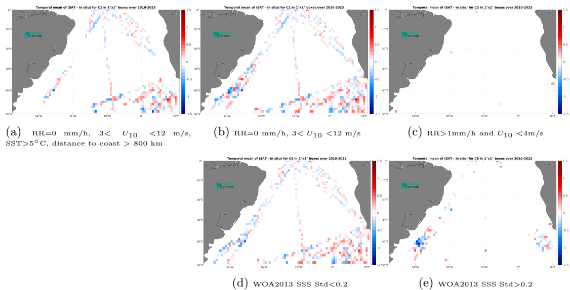
Figure 14: Temporal mean gridded over spatial boxes of size 1^\circ \times 1^\circ of \Delta\text{SSS} (SMOS SSS L3 v335 - Monthly - 25 km (CATDS-CPDC) - TSG (Polarstern)) for 5 different subdatasets corresponding to:RR=0 mm/h, 3 < U_{10} < 12 m/s, SST >5^\circ\text{C} , distance to coast > 800 km (a), RR=0 mm/h, 3 < U_{10} < 12 m/s (b), RR >1 mm/h and U_{10} < 4 m/s (c), WOA2013 SSS Std <0.2 (d), WOA2013 SSS Std >0.2 (e).
