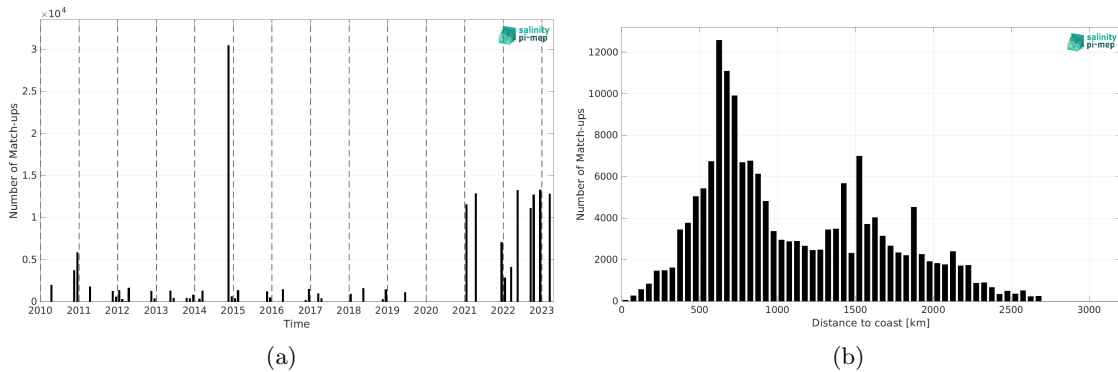
Figure 2: Number of match-ups between TSG (Polarstern) and SMOS SSS L3 v335 - Monthly - 25 km (CATDS-CPDC) SSS as a function of time (a) and as function of the distance to coast (b) over the South Atlantic Ocean Pi-MEP region and for the full satellite product period.
