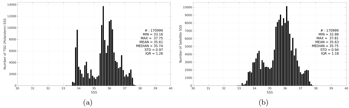
Figure 3: Histograms of SSS from TSG (Polarstern) (a) and SMOS SSS L3 v335 - Monthly - 25 km (CATDS-CPDC) (b) considering all match-up pairs per bins of 0.1 over the South Atlantic Ocean Pi-MEP region and for the full satellite product period.
