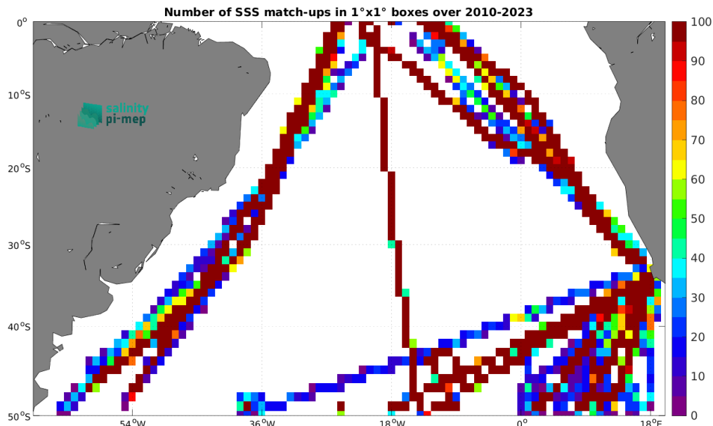
Figure 5: Number of SSS match-ups between TSG (Polarstern) SSS and the SMOS SSS L3 v335 - Monthly - 25 km (CATDS-CPDC) SSS product for the South Atlantic Ocean Pi-MEP region over 1^\circ \times 1^\circ boxes and for the full satellite product period.
