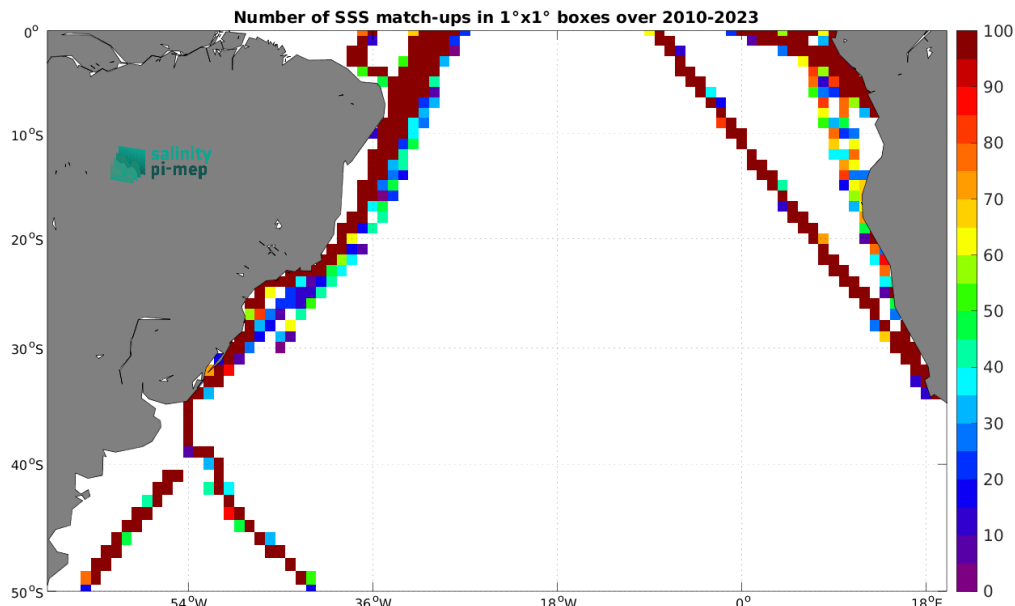
Figure 5: Number of SSS match-ups between TSG (LEGOS-DM) SSS and the SMOS SSS L3 v335 - Monthly - 25 km (CATDS-CPDC) SSS product for the South Atlantic Ocean Pi-MEP region over 1^\circ \times 1^\circ boxes and for the full satellite product period.
