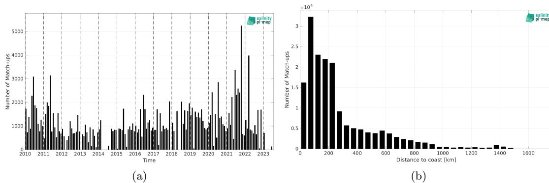
Figure 2: Number of match-ups between TSG (LEGOS-DM) and SMOS SSS L3 v335 - Monthly - 25 km (CATDS-CPDC) SSS as a function of time (a) and as function of the distance to coast (b) over the South Atlantic Ocean Pi-MEP region and for the full satellite product period.
