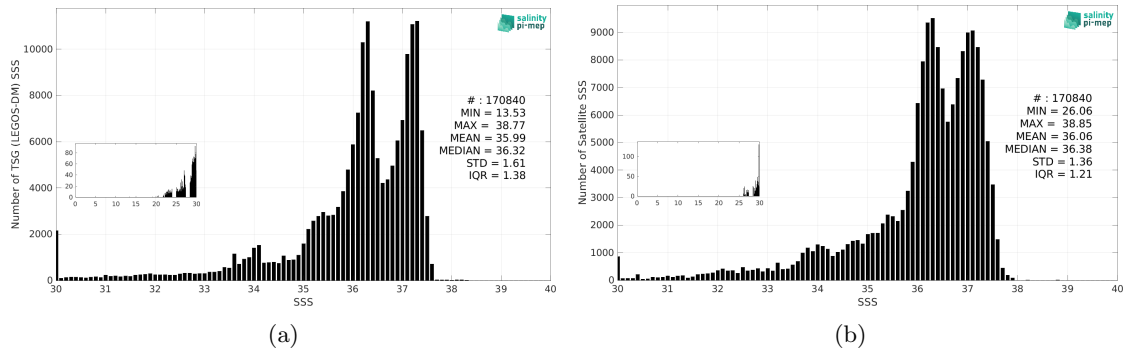
Figure 3: Histograms of SSS from TSG (LEGOS-DM) (a) and SMOS SSS L3 v335 - Monthly - 25 km (CATDS-CPDC) (b) considering all match-up pairs per bins of 0.1 over the South Atlantic Ocean Pi-MEP region and for the full satellite product period.
