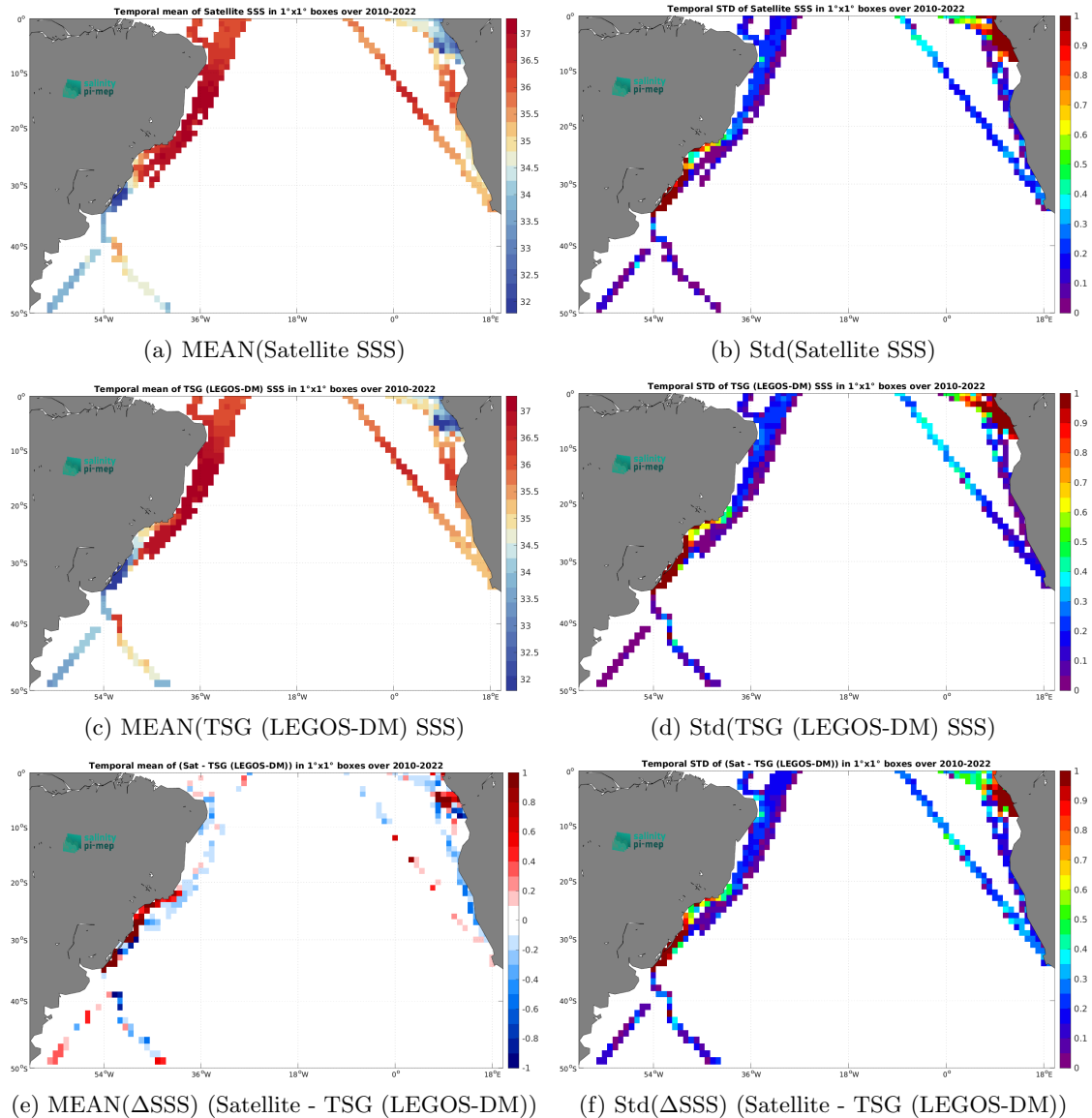
Figure 7: Temporal mean (left) and Std (right) of SSS from SMOS SSS L3 v335 - Monthly - 25 km (CATDS-CPDC) (top), TSG (LEGOS-DM) (middle), and of \Delta SSS (Satellite - TSG (LEGOS-DM)). Only match-up pairs are used to generate these maps.
