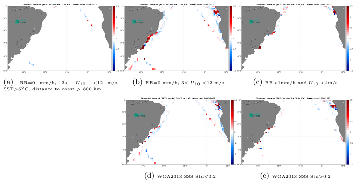
Figure 14: Temporal mean gridded over spatial boxes of size 1^\circ \times 1^\circ of \Delta\text{SSS} (SMOS SSS L3 v335 - Monthly - 25 km (CATDS-CPDC) - TSG (LEGOS-DM)) for 5 different subdatasets corresponding to:RR=0 mm/h, 3 < U_{10} < 12 m/s, SST >5^\circ\text{C} , distance to coast > 800 km (a), RR=0 mm/h, 3 < U_{10} < 12 m/s (b), RR >1 mm/h and U_{10} < 4 m/s (c), WOA2013 SSS Std <0.2 (d), WOA2013 SSS Std >0.2 (e).
