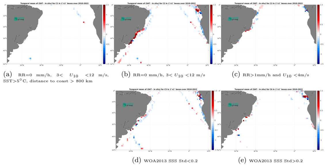
Figure 12: Temporal mean gridded over spatial boxes of size 1^\circ \times 1^\circ of \Delta SSS (SMOS SSS L3 v335 - Monthly - 25 km (CATDS-CPDC) - TSG (LEGOS-DM)) for 5 different subdatasets corresponding to:RR=0 mm/h, 3 < U_{10} < 12 m/s, SST >5^\circ\text{C} , distance to coast > 800 km (a), RR=0 mm/h, 3 < U_{10} < 12 m/s (b), RR >1 mm/h and U_{10} < 4 m/s (c), WOA2013 SSS Std <0.2 (d), WOA2013 SSS Std >0.2 (e).
