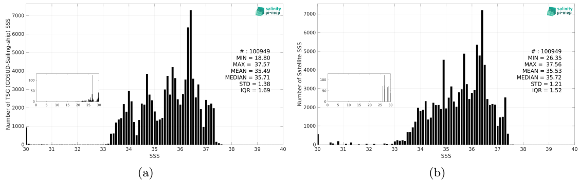
Figure 3: Histograms of SSS from TSG (GOSUD-Sailing-ship) (a) and SMOS SSS L3 v335 - Monthly - 25 km (CATDS-CPDC) (b) considering all match-up pairs per bins of 0.1 over the South Atlantic Ocean Pi-MEP region and for the full satellite product period.
