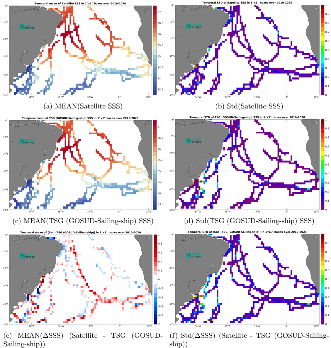
Figure 7: Temporal mean (left) and Std (right) of SSS from SMOS SSS L3 v335 - Monthly - 25 km (CATDS-CPDC) (top), TSG (GOSUD-Sailing-ship) (middle), and of \Delta SSS (Satellite - TSG (GOSUD-Sailing-ship)). Only match-up pairs are used to generate these maps.
