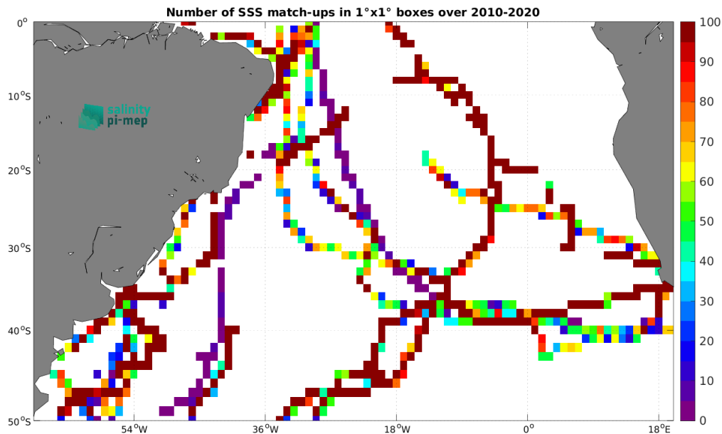
Figure 5: Number of SSS match-ups between TSG (GOSUD-Sailing-ship) SSS and the SMOS SSS L3 v335 - Monthly - 25 km (CATDS-CPDC) SSS product for the South Atlantic Ocean Pi-MEP region over 1^\circ \times 1^\circ boxes and for the full satellite product period.
