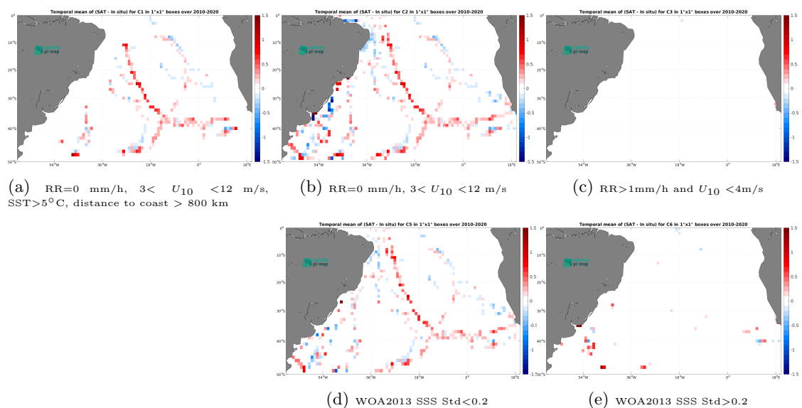
Figure 14: Temporal mean gridded over spatial boxes of size 1^\circ \times 1^\circ of \Delta\text{SSS} (SMOS SSS L3 v335 - Monthly - 25 km (CATDS-CPDC) - TSG (GOSUD-Sailing-ship)) for 5 different subdatasets corresponding to:RR=0 mm/h, 3 < U_{10} < 12 m/s, SST >5^\circ\text{C} , distance to coast > 800 km (a), RR=0 mm/h, 3 < U_{10} < 12 m/s (b), RR >1 mm/h and U_{10} < 4 m/s (c), WOA2013 SSS Std <0.2 (d), WOA2013 SSS Std >0.2 (e).
