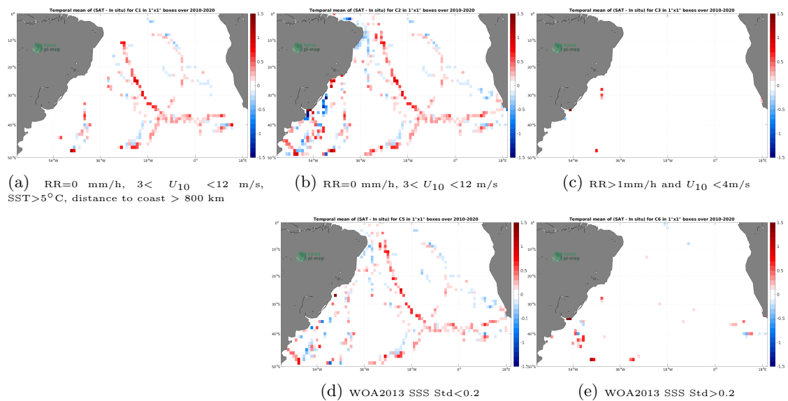
Figure 12: Temporal mean gridded over spatial boxes of size 1^\circ \times 1^\circ of \Delta\text{SSS} (SMOS SSS L3 v335 - Monthly - 25 km (CATDS-CPDC) - TSG (GOSUD-Sailing-ship)) for 5 different subdatasets corresponding to:RR=0 mm/h, 3 < U_{10} < 12 m/s, SST >5^\circ\text{C} , distance to coast > 800 km (a), RR=0 mm/h, 3 < U_{10} < 12 m/s (b), RR >1 mm/h and U_{10} < 4 m/s (c), WOA2013 SSS Std <0.2 (d), WOA2013 SSS Std >0.2 (e).
