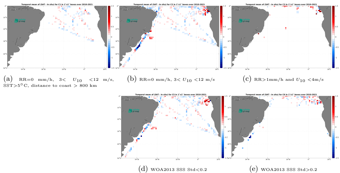
Figure 12: Temporal mean gridded over spatial boxes of size 1^\circ \times 1^\circ of \Delta\text{SSS} (SMOS SSS L3 v335 - Monthly - 25 km (CATDS-CPDC) - TSG (GOSUD-Research-vessel)) for 5 different subdatasets corresponding to:RR=0 mm/h, 3 < U_{10} < 12 m/s, SST >5^\circ\text{C} , distance to coast > 800 km (a), RR=0 mm/h, 3 < U_{10} < 12 m/s (b), RR >1 mm/h and U_{10} < 4 m/s (c), WOA2013 SSS Std <0.2 (d), WOA2013 SSS Std >0.2 (e).
