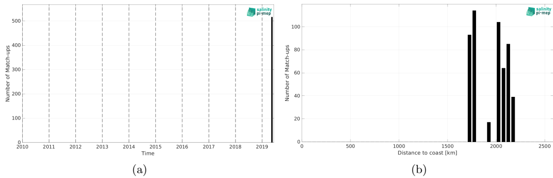
Figure 2: Number of match-ups between Saildrone and SMOS SSS L3 v335 - Monthly - 25 km (CATDS-CPDC) SSS as a function of time (a) and as function of the distance to coast (b) over the South Atlantic Ocean Pi-MEP region and for the full satellite product period.
