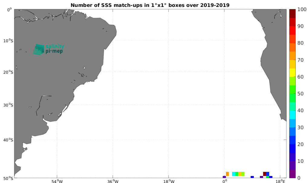
Figure 5: Number of SSS match-ups between Sairdrone SSS and the SMOS SSS L3 v335 - Monthly - 25 km (CATDS-CPDC) SSS product for the South Atlantic Ocean Pi-MEP region over 1^\circ \times 1^\circ boxes and for the full satellite product period.
