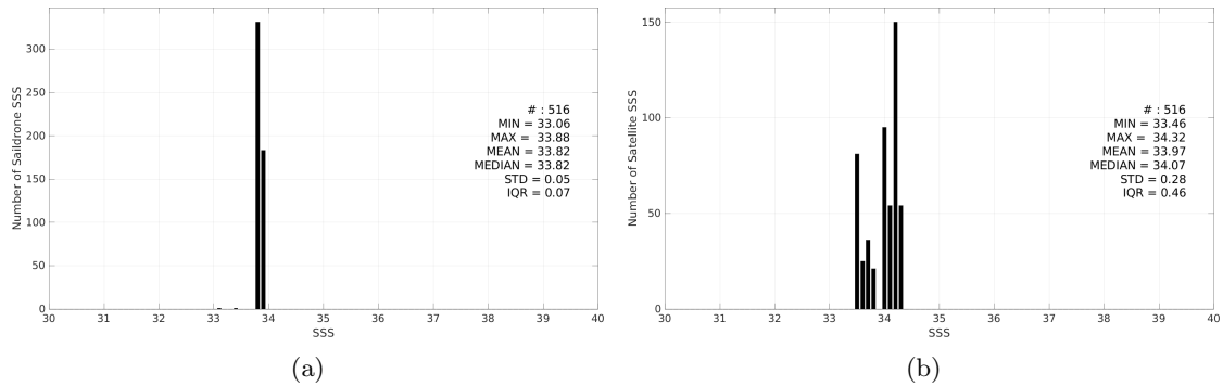
Figure 3: Histograms of SSS from Sailability (a) and SMOS SSS L3 v335 - Monthly - 25 km (CATDS-CPDC) (b) considering all match-up pairs per bins of 0.1 over the South Atlantic Ocean Pi-MEP region and for the full satellite product period.
