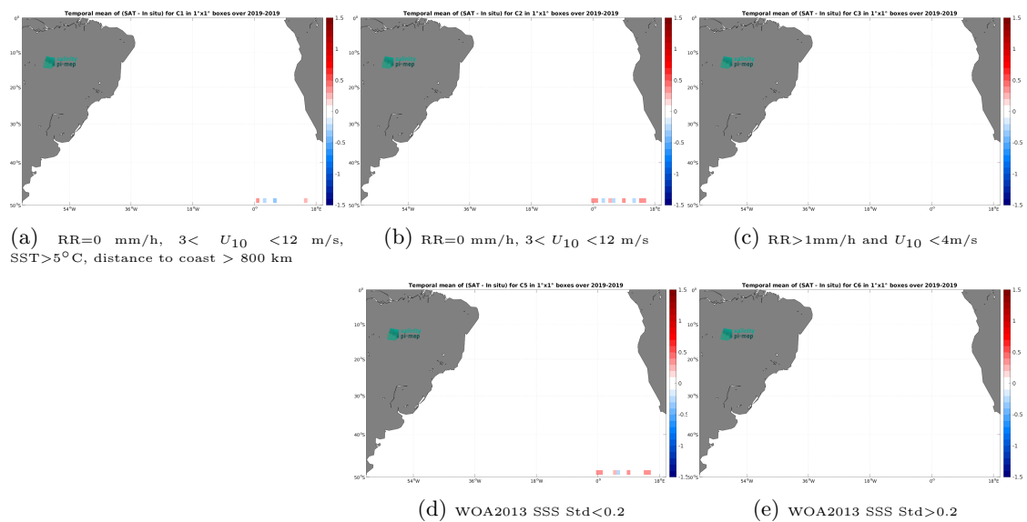
Figure 14: Temporal mean gridded over spatial boxes of size 1^\circ \times 1^\circ of \Delta SSS (SMOS SSS L3 v335 - Monthly - 25 km (CATDS-CPDC) - Sailability) for 5 different subdatasets corresponding to:RR=0 mm/h, 3 < U_{10} < 12 m/s, SST >5^\circ\text{C} , distance to coast > 800 km (a), RR=0 mm/h, 3 < U_{10} < 12 m/s (b), RR >1 mm/h and U_{10} < 4 m/s (c), WOA2013 SSS Std <0.2 (d), WOA2013 SSS Std >0.2 (e).
