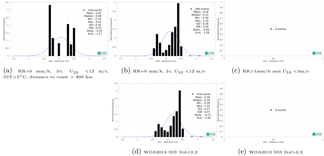
Figure 15: Normalized histogram of \Delta SSS (SMOS SSS L3 v335 - Monthly - 25 km (CATDS-CPDC) - Saildrone) for 5 different subdatasets corresponding to: RR=0 mm/h, 3 < U_{10} < 12 m/s, SST > 5°C, distance to coast > 800 km (a), RR=0 mm/h, 3 < U_{10} < 12 m/s (b), RR > 1mm/h and U_{10} < 4 m/s (c), WOA2013 SSS Std < 0.2 (d), WOA2013 SSS Std > 0.2 (e).
