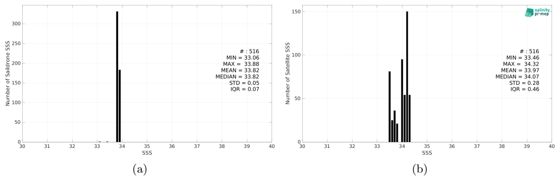
Figure 2: Histograms of SSS from Saildrone (a) and SMOS SSS L3 v335 - Monthly - 25 km (CATDS-CPDC) (b) considering all match-up pairs per bins of 0.1 over the South Atlantic Ocean Pi-MEP region and for the full satellite product period.
