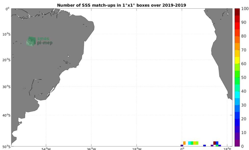
Figure 4: Number of SSS match-ups between Sairdrone SSS and the SMOS SSS L3 v335 - Monthly - 25 km (CATDS-CPDC) SSS product for the South Atlantic Ocean Pi-MEP region over 1^\circ \times 1^\circ boxes and for the full satellite product period.
