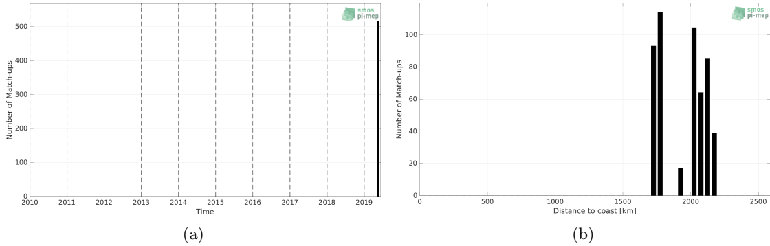
Figure 1: Number of match-ups between Saildrone and SMOS SSS L3 v335 - Monthly - 25 km (CATDS-CPDC) SSS as a function of time (a) and as function of the distance to coast (b) over the South Atlantic Ocean Pi-MEP region and for the full satellite product period.
