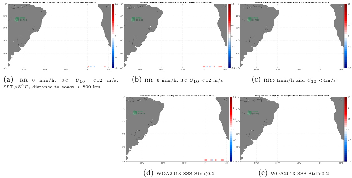
Figure 12: Temporal mean gridded over spatial boxes of size 1^{\circ}\times 1^{\circ} of \Delta\text{SSS} (SMOS SSS L3 v335 - Monthly - 25 km (CATDS-CPDC) - Saildrone) for 5 different subdatasets corresponding to:RR=0 mm/h, 3 < U_{10} < 12 m/s, SST >5^{\circ}\text{C} , distance to coast > 800 km (a), RR=0 mm/h, 3 < U_{10} < 12 m/s (b), RR >1 mm/h and U_{10} < 4 m/s (c), WOA2013 SSS Std <0.2 (d), WOA2013 SSS Std >0.2 (e).
