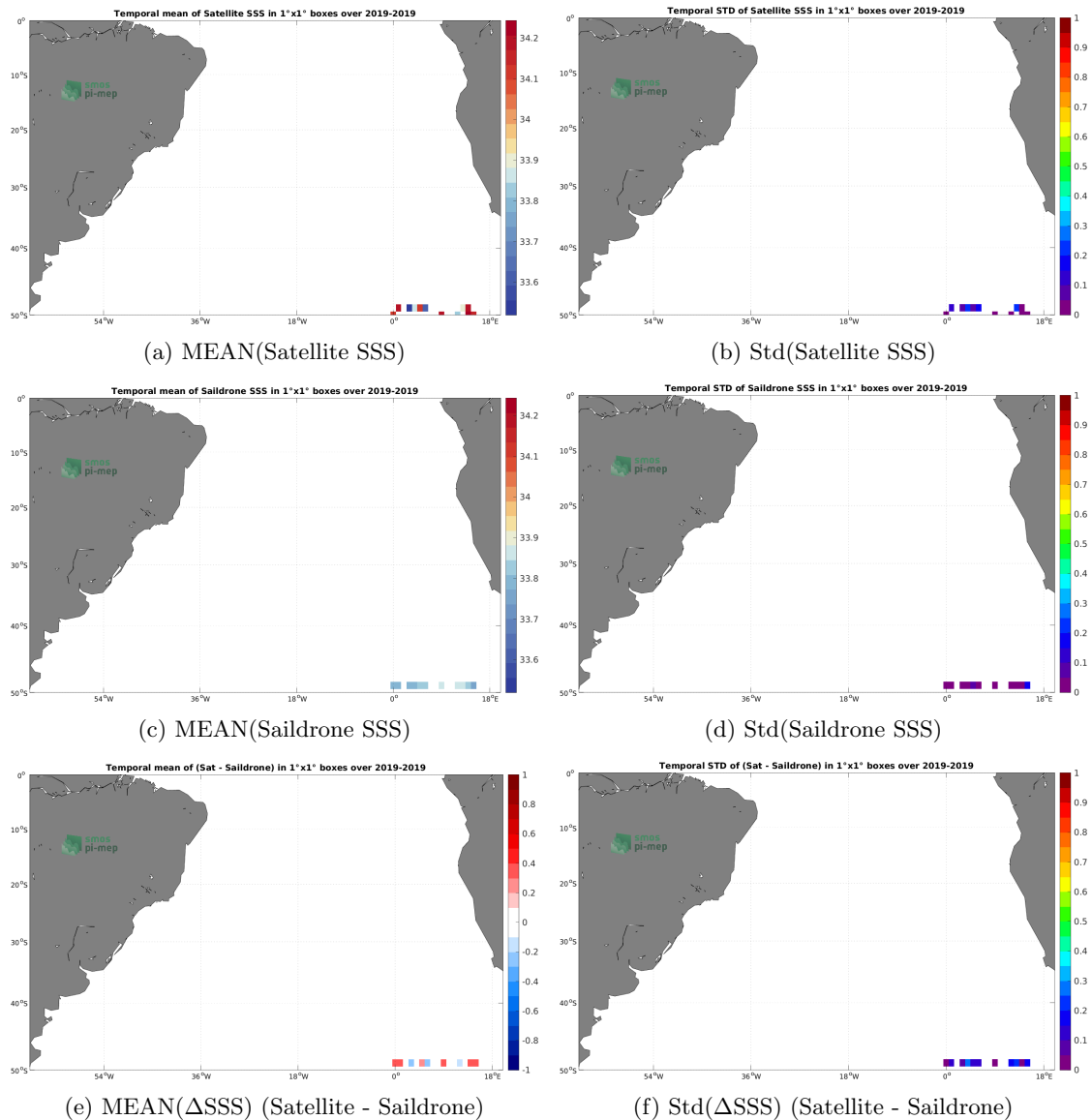
Figure 6: Temporal mean (left) and Std (right) of SSS from SMOS SSS L3 v335 - Monthly - 25 km (CATDS-CPDC) (top), Saildrone (middle), and of \Delta SSS (Satellite - Saildrone). Only match-up pairs are used to generate these maps.
