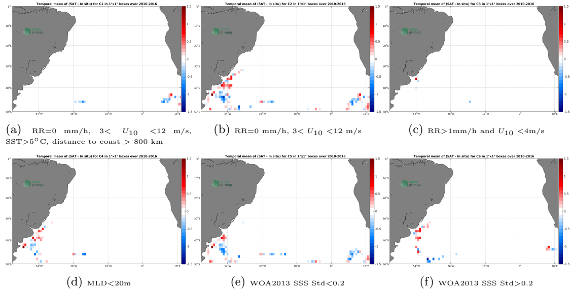
Figure 12: Temporal mean gridded over spatial boxes of size 1^\circ \times 1^\circ of \Delta SSS (SMOS SSS L3 v335 - Monthly - 25 km (CATDS-CPDC) - Marine mammals) for 6 different subdatasets corresponding to: RR=0 mm/h, 3 < U_{10} < 12 m/s, SST > 5^\circ C , distance to coast > 800 km (a), RR=0 mm/h, 3 < U_{10} < 12 m/s (b), RR > 1 mm/h and U_{10} < 4 m/s (c), MLD < 20 m (d), WOA2013 SSS Std < 0.2 (e), WOA2013 SSS Std > 0.2 (f).
