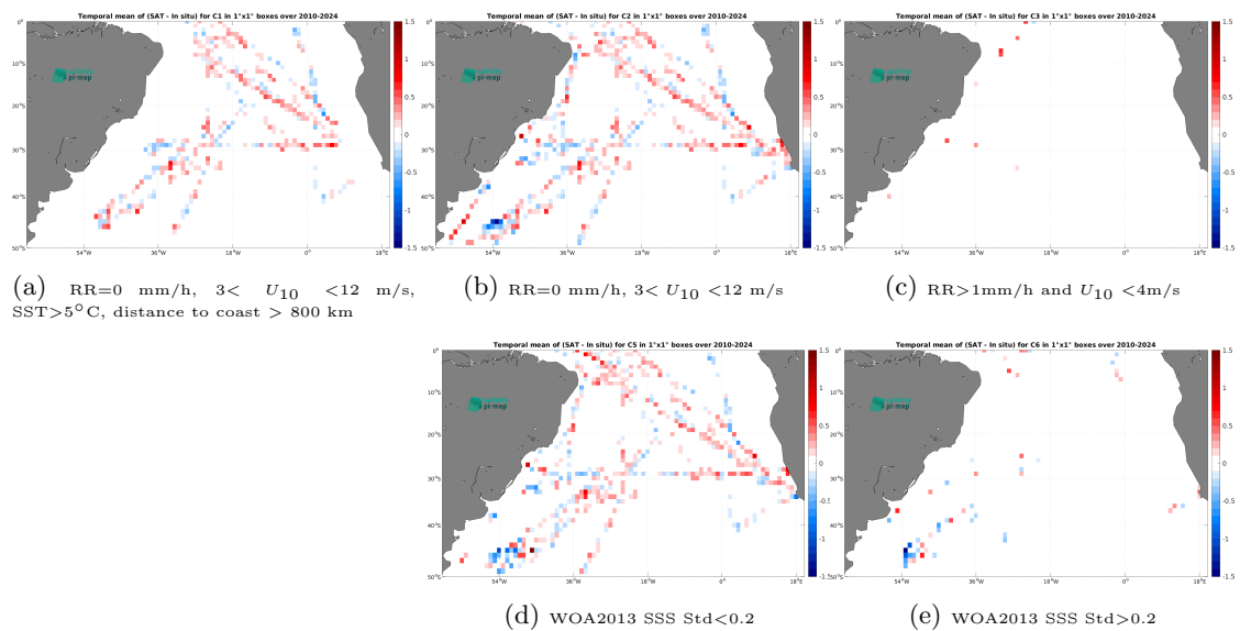
Figure 14: Temporal mean gridded over spatial boxes of size 1^\circ \times 1^\circ of \Delta\text{SSS} (SMOS SSS L3 v335 - 10 Days - 25 km (CATDS-CPDC) - TSG (SAMOS)) for 5 different subdatasets corresponding to:RR=0 mm/h, 3 < U_{10} < 12 m/s, SST >5^\circ\text{C} , distance to coast > 800 km (a), RR=0 mm/h, 3 < U_{10} < 12 m/s (b), RR >1 mm/h and U_{10} < 4 m/s (c), WOA2013 SSS Std <0.2 (d), WOA2013 SSS Std >0.2 (e).
