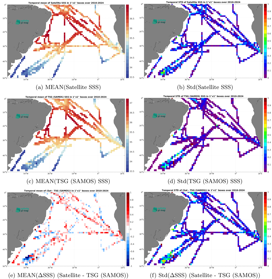
Figure 7: Temporal mean (left) and Std (right) of SSS from SMOS SSS L3 v335 - 10 Days - 25 km (CATDS-CPDC) (top), TSG (SAMOS) (middle), and of \Delta SSS (Satellite - TSG (SAMOS)). Only match-up pairs are used to generate these maps.
