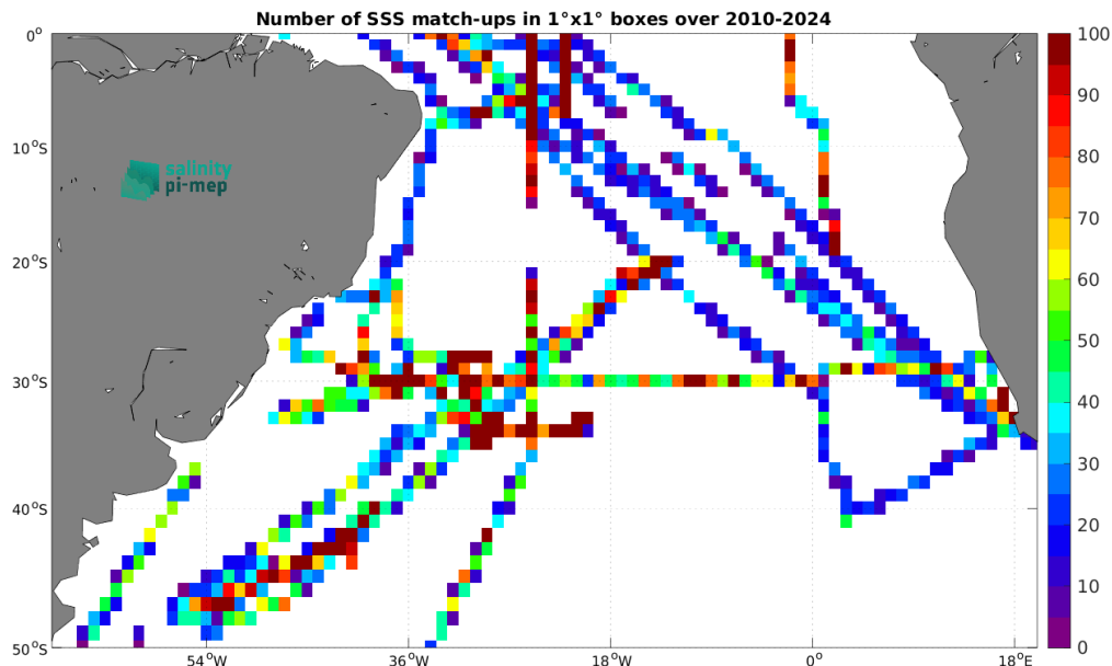
Figure 5: Number of SSS match-ups between TSG (SAMOS) SSS and the SMOS SSS L3 v335 - 10 Days - 25 km (CATDS-CPDC) SSS product for the South Atlantic Ocean Pi-MEP region over 1^\circ \times 1^\circ boxes and for the full satellite product period.
