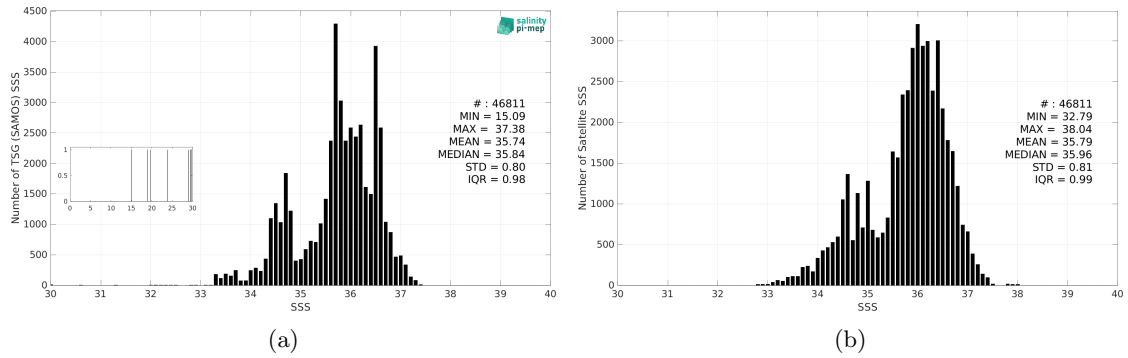
Figure 3: Histograms of SSS from TSG (SAMOS) (a) and SMOS SSS L3 v335 - 10 Days - 25 km (CATDS-CPDC) (b) considering all match-up pairs per bins of 0.1 over the South Atlantic Ocean Pi-MEP region and for the full satellite product period.
