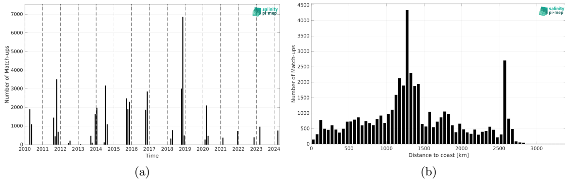
Figure 2: Number of match-ups between TSG (SAMOS) and SMOS SSS L3 v335 - 10 Days - 25 km (CATDS-CPDC) SSS as a function of time (a) and as function of the distance to coast (b) over the South Atlantic Ocean Pi-MEP region and for the full satellite product period.
