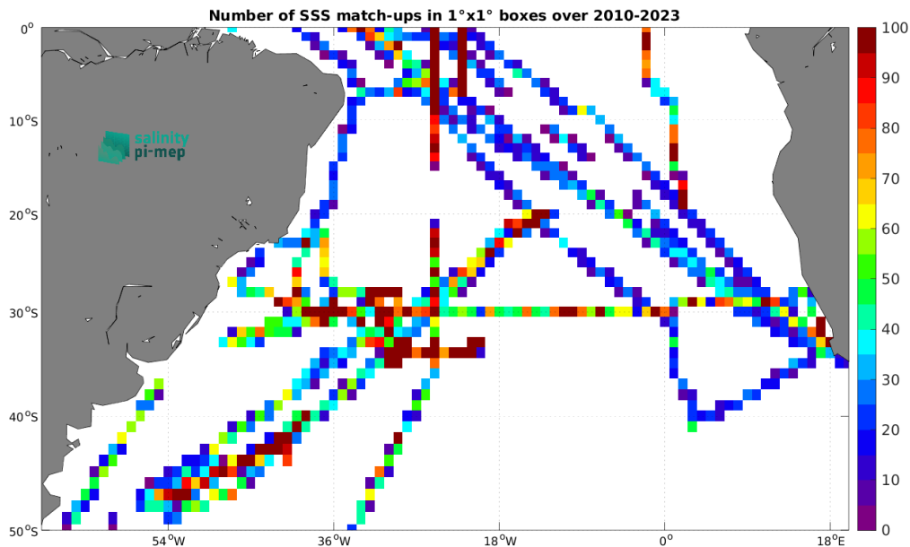
Figure 4: Number of SSS match-ups between TSG (SAMOS) SSS and the SMOS SSS L3 v335 - 10 Days - 25 km (CATDS-CPDC) SSS product for the South Atlantic Ocean Pi-MEP region over 1^\circ \times 1^\circ boxes and for the full satellite product period.
