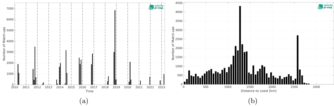
Figure 1: Number of match-ups between TSG (SAMOS) and SMOS SSS L3 v335 - 10 Days - 25 km (CATDS-CPDC) SSS as a function of time (a) and as function of the distance to coast (b) over the South Atlantic Ocean Pi-MEP region and for the full satellite product period.
