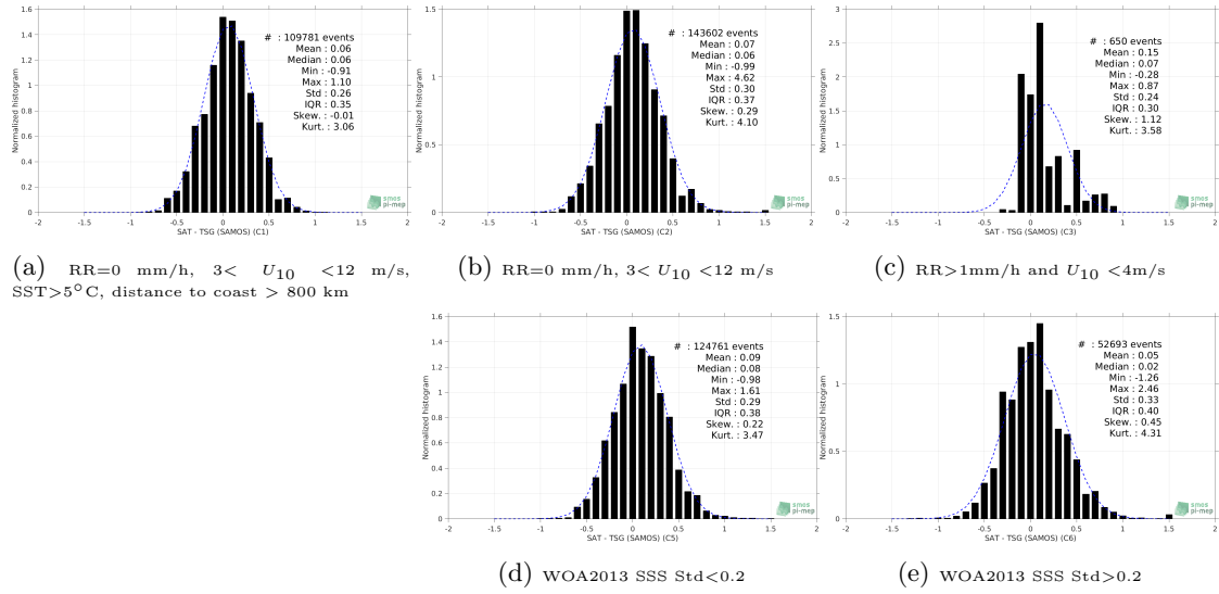
Figure 13: Normalized histogram of \Delta\text{SSS} (SMOS SSS L3 v335 - 10 Days - 25 km (CATDS-CPDC) - TSG (SAMOS)) for 5 different subdatasets corresponding to: RR=0 mm/h, 3 < U_{10} < 12 m/s, SST>5°C, distance to coast > 800 km (a), RR=0 mm/h, 3 < U_{10} < 12 m/s (b), RR>1mm/h and U_{10} < 4 m/s (c), WOA2013 SSS Std<0.2 (d), WOA2013 SSS Std>0.2 (e).
