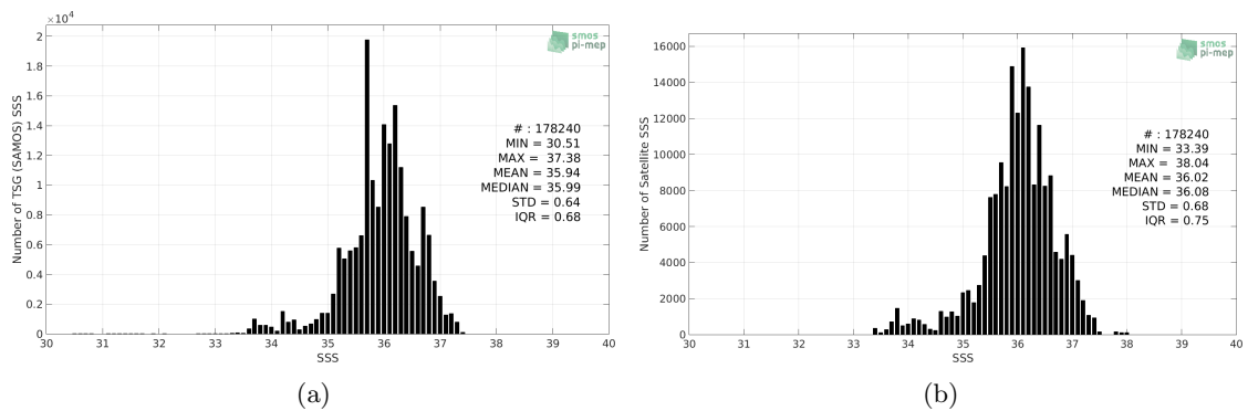
Figure 2: Histograms of SSS from TSG (SAMOS) (a) and SMOS SSS L3 v335 - 10 Days - 25 km (CATDS-CPDC) (b) considering all match-up pairs per bins of 0.1 over the South Atlantic Ocean Pi-MEP region and for the full satellite product period.
