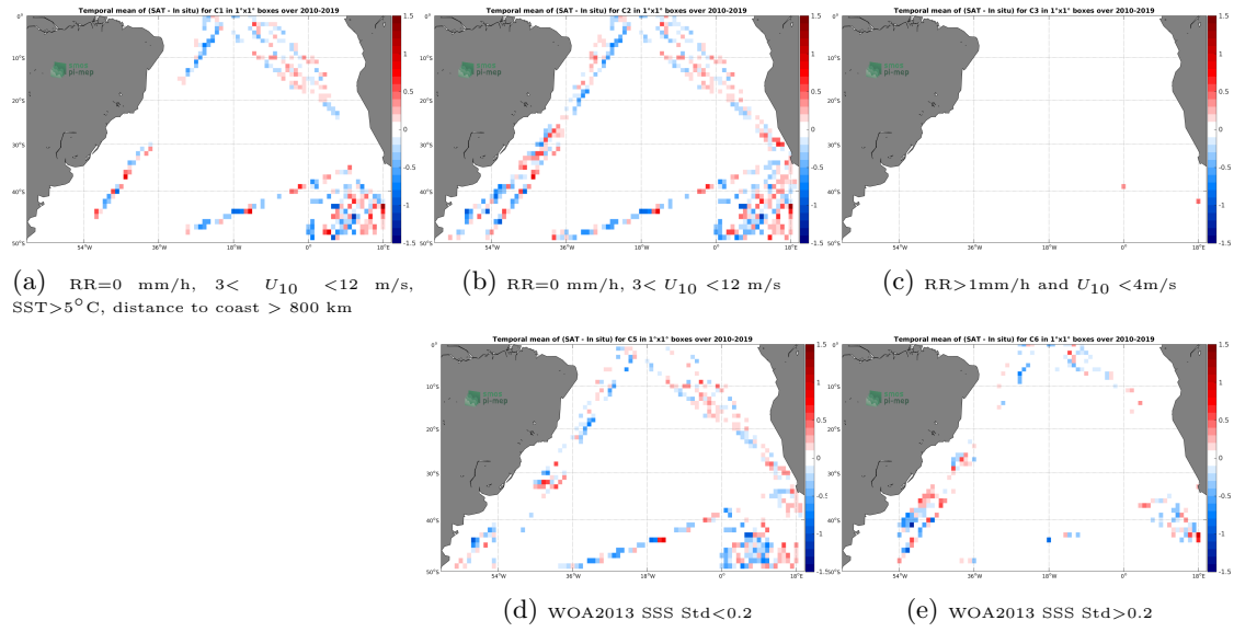
Figure 12: Temporal mean gridded over spatial boxes of size 1^\circ \times 1^\circ of \Delta\text{SSS} (SMOS SSS L3 v335 - 10 Days - 25 km (CATDS-CPDC) - TSG (Polarstern)) for 5 different subdatasets corresponding to: \text{RR}=0 mm/h, 3 < U_{10} < 12 m/s, \text{SST} > 5^\circ\text{C} , distance to coast > 800 km (a), \text{RR}=0 mm/h, 3 < U_{10} < 12 m/s (b), \text{RR} > 1 mm/h and U_{10} < 4 m/s (c), WOA2013 SSS Std < 0.2 (d), WOA2013 SSS Std > 0.2 (e).
