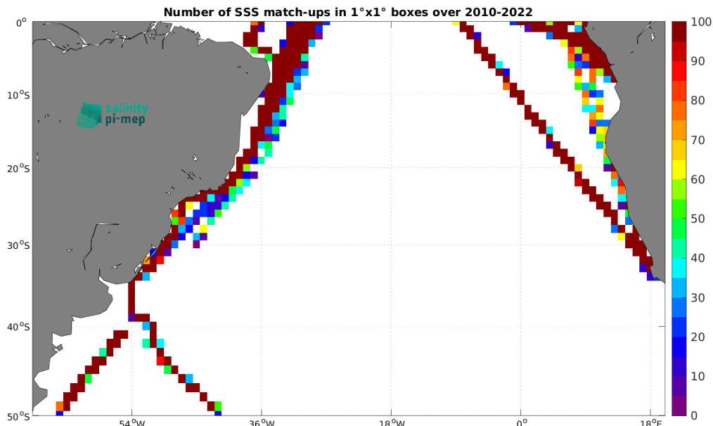
Figure 5: Number of SSS match-ups between TSG (LEGOS-DM) SSS and the SMOS SSS L3 v335 - 10 Days - 25 km (CATDS-CPDC) SSS product for the South Atlantic Ocean Pi-MEP region over 1^\circ \times 1^\circ boxes and for the full satellite product period.
