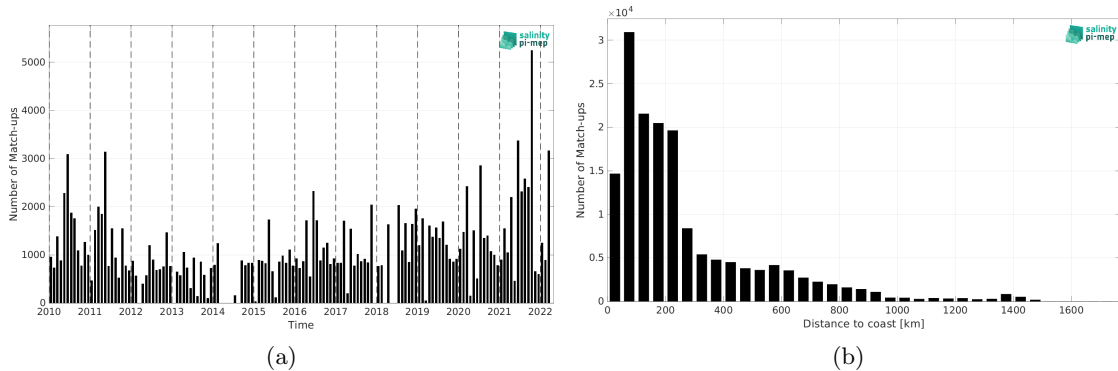
Figure 2: Number of match-ups between TSG (LEGOS-DM) and SMOS SSS L3 v335 - 10 Days - 25 km (CATDS-CPDC) SSS as a function of time (a) and as function of the distance to coast (b) over the South Atlantic Ocean Pi-MEP region and for the full satellite product period.
