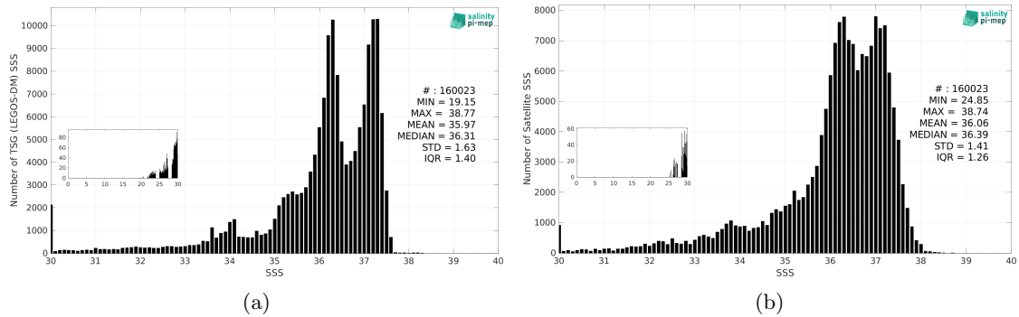
Figure 3: Histograms of SSS from TSG (LEGOS-DM) (a) and SMOS SSS L3 v335 - 10 Days - 25 km (CATDS-CPDC) (b) considering all match-up pairs per bins of 0.1 over the South Atlantic Ocean Pi-MEP region and for the full satellite product period.
