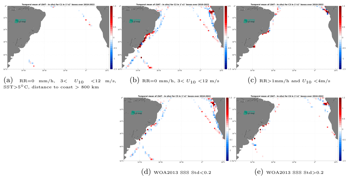
Figure 14: Temporal mean gridded over spatial boxes of size 1^\circ \times 1^\circ of \Delta SSS (SMOS SSS L3 v335 - 10 Days - 25 km (CATDS-CPDC) - TSG (LEGOS-DM)) for 5 different subdatasets corresponding to:RR=0 mm/h, 3 < U_{10} < 12 m/s, SST >5^\circ\text{C} , distance to coast > 800 km (a), RR=0 mm/h, 3 < U_{10} < 12 m/s (b), RR >1 mm/h and U_{10} < 4 m/s (c), WOA2013 SSS Std <0.2 (d), WOA2013 SSS Std >0.2 (e).
