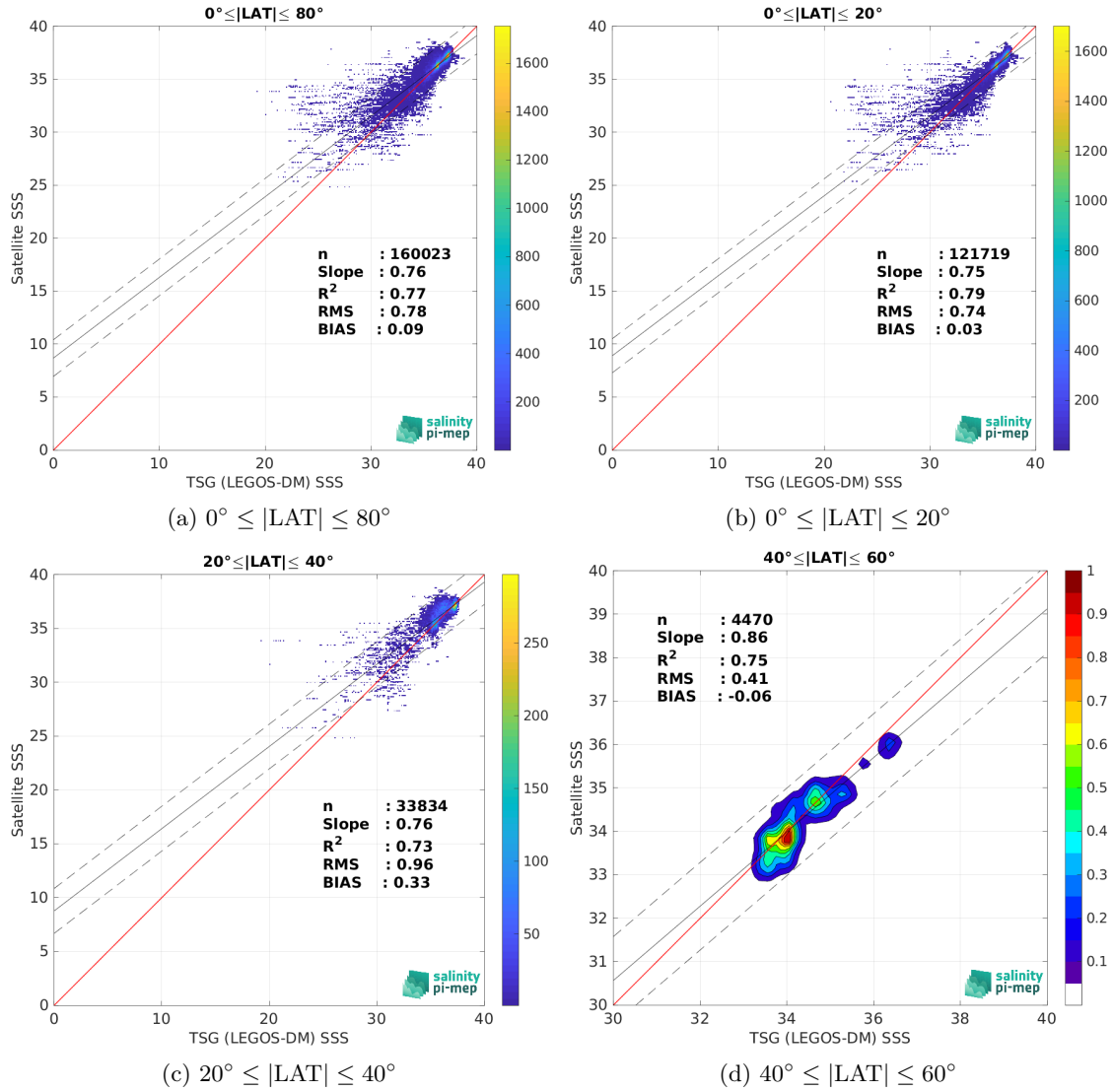
Figure 10: Contour maps of the concentration of SMOS SSS L3 v335 - 10 Days - 25 km (CATDS-CPDC) SSS (y-axis) versus TSG (LEGOS-DM) SSS (x-axis) at match-up pairs for different latitude bands. For each plot, the red line shows x=y . The black thin and dashed lines indicate a linear fit through the data cloud and the \pm 95\% confidence levels, respectively. The number of match-up pairs n , the slope and R^2 coefficient of the linear fit, the root mean square (RMS) and the mean bias between satellite and in situ data are indicated for each latitude band in each plot.
