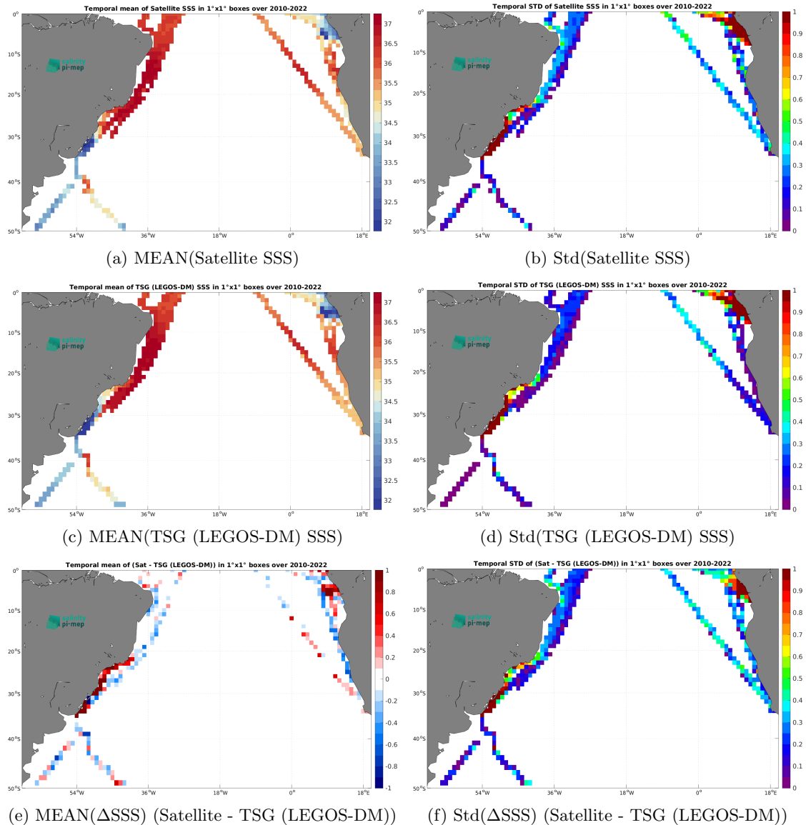
Figure 7: Temporal mean (left) and Std (right) of SSS from SMOS SSS L3 v335 - 10 Days - 25 km (CATDS-CPDC) (top), TSG (LEGOS-DM) (middle), and of \Delta SSS (Satellite - TSG (LEGOS-DM)). Only match-up pairs are used to generate these maps.
