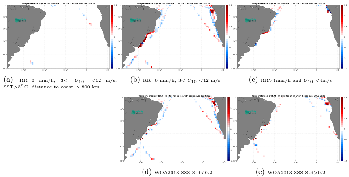
Figure 12: Temporal mean gridded over spatial boxes of size 1^\circ \times 1^\circ of \Delta SSS (SMOS SSS L3 v335 - 10 Days - 25 km (CATDS-CPDC) - TSG (LEGOS-DM)) for 5 different subdatasets corresponding to:RR=0 mm/h, 3 < U_{10} < 12 m/s, SST >5^\circ\text{C} , distance to coast > 800 km (a), RR=0 mm/h, 3 < U_{10} < 12 m/s (b), RR >1 mm/h and U_{10} < 4 m/s (c), WOA2013 SSS Std <0.2 (d), WOA2013 SSS Std >0.2 (e).
