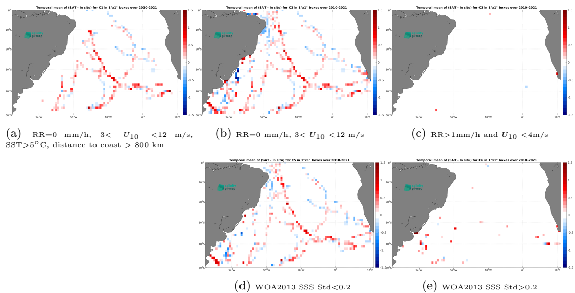
Figure 14: Temporal mean gridded over spatial boxes of size 1^\circ \times 1^\circ of \Delta\text{SSS} (SMOS SSS L3 v335 - 10 Days - 25 km (CATDS-CPDC) - TSG (GOSUD-Sailing-ship)) for 5 different subdatasets corresponding to:RR=0 mm/h, 3 < U_{10} < 12 m/s, SST >5^\circ\text{C} , distance to coast > 800 km (a), RR=0 mm/h, 3 < U_{10} < 12 m/s (b), RR >1 mm/h and U_{10} < 4 m/s (c), WOA2013 SSS Std <0.2 (d), WOA2013 SSS Std >0.2 (e).
