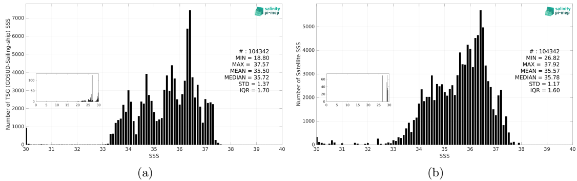
Figure 3: Histograms of SSS from TSG (GOSUD-Sailing-ship) (a) and SMOS SSS L3 v335 - 10 Days - 25 km (CATDS-CPDC) (b) considering all match-up pairs per bins of 0.1 over the South Atlantic Ocean Pi-MEP region and for the full satellite product period.
