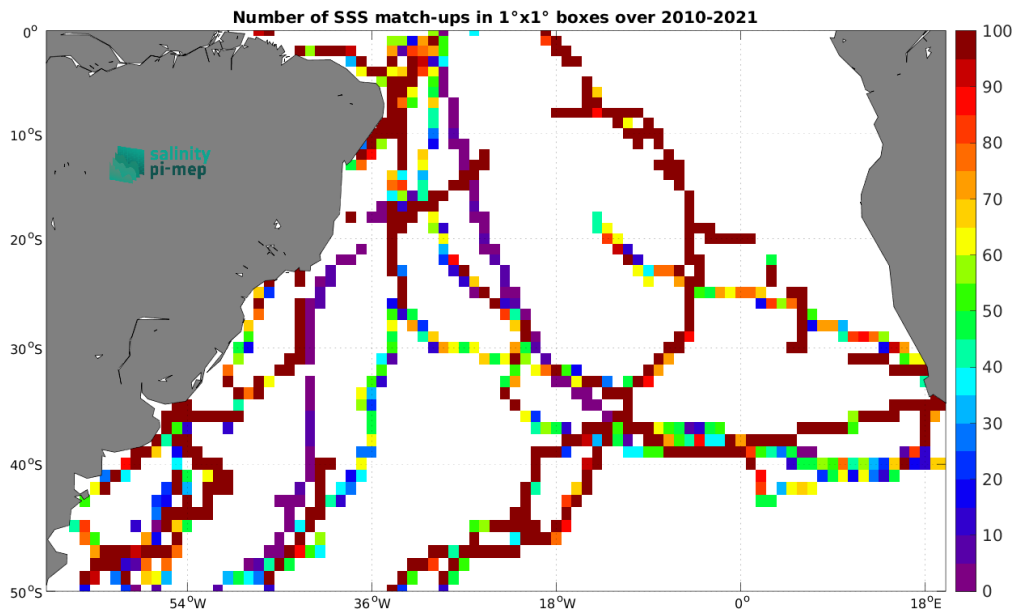
Figure 5: Number of SSS match-ups between TSG (GOSUD-Sailing-ship) SSS and the SMOS SSS L3 v335 - 10 Days - 25 km (CATDS-CPDC) SSS product for the South Atlantic Ocean Pi-MEP region over 1^\circ \times 1^\circ boxes and for the full satellite product period.
