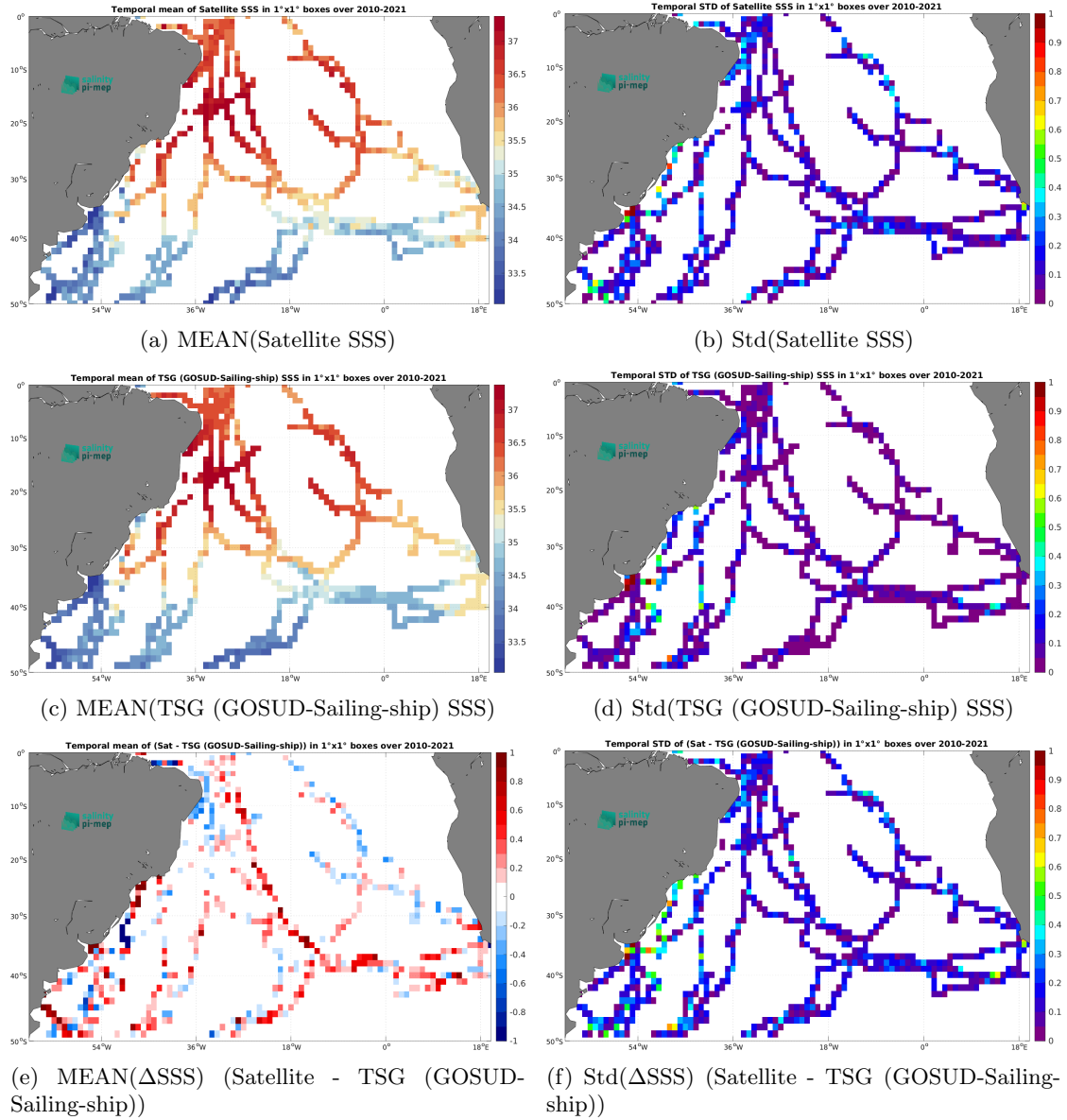
Figure 7: Temporal mean (left) and Std (right) of SSS from SMOS SSS L3 v335 - 10 Days - 25 km (CATDS-CPDC) (top), TSG (GOSUD-Sailing-ship) (middle), and of \Delta SSS (Satellite - TSG (GOSUD-Sailing-ship)). Only match-up pairs are used to generate these maps.
