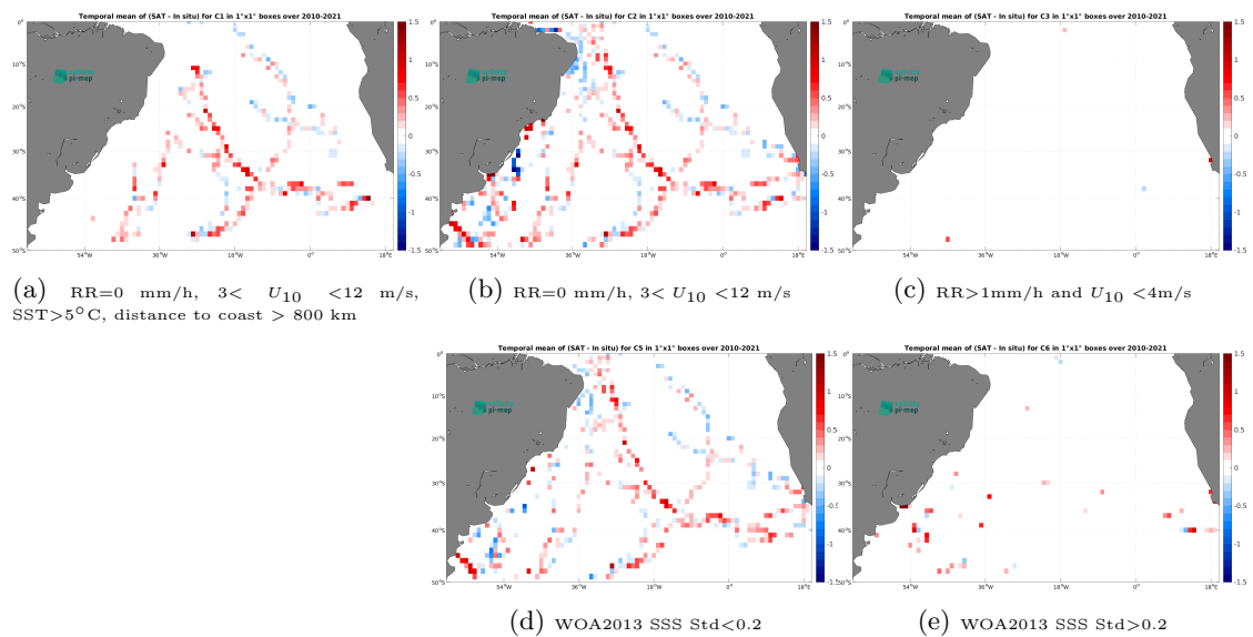
Figure 14: Temporal mean gridded over spatial boxes of size 1^\circ \times 1^\circ of \Delta SSS (SMOS SSS L3 v335 - 10 Days - 25 km (CATDS-CPDC) - TSG (GOSUD-Sailing-ship)) for 5 different subdatasets corresponding to:RR=0 mm/h, 3 < U_{10} < 12 m/s, SST>5°C, distance to coast > 800 km (a), RR=0 mm/h, 3 < U_{10} < 12 m/s (b), RR>1mm/h and U_{10} < 4 m/s (c), WOA2013 SSS Std<0.2 (d), WOA2013 SSS Std>0.2 (e).
