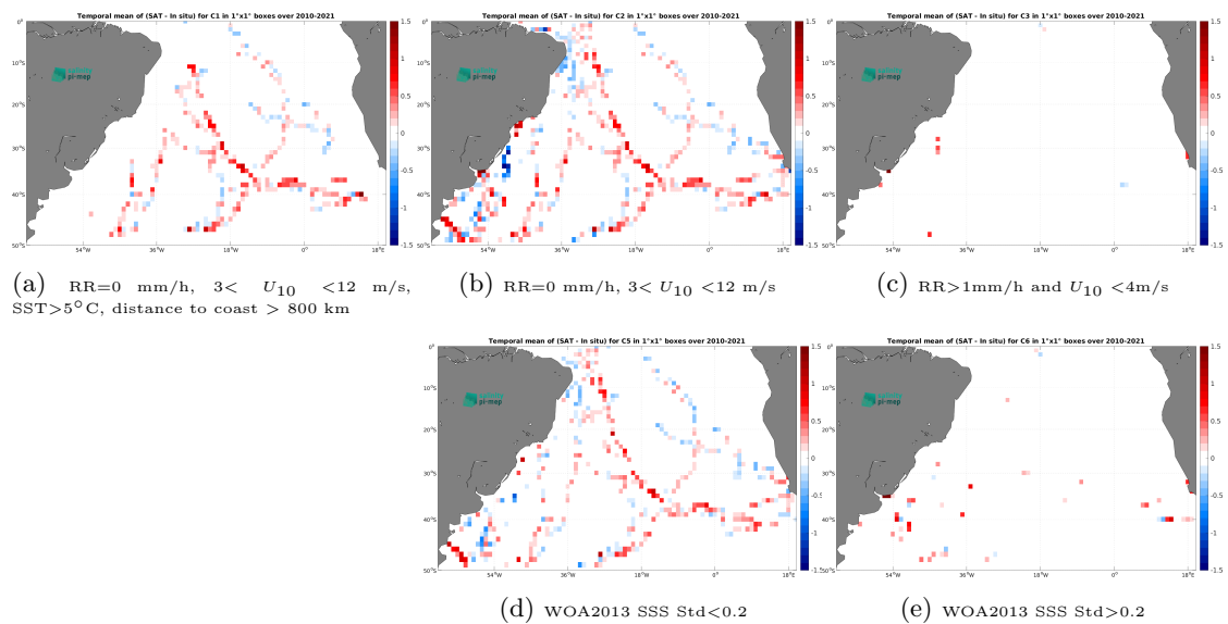
Figure 12: Temporal mean gridded over spatial boxes of size 1^\circ \times 1^\circ of \Delta\text{SSS} (SMOS SSS L3 v335 - 10 Days - 25 km (CATDS-CPDC) - TSG (GOSUD-Sailing-ship)) for 5 different subdatasets corresponding to:RR=0 mm/h, 3 < U_{10} < 12 m/s, SST >5^\circ\text{C} , distance to coast > 800 km (a), RR=0 mm/h, 3 < U_{10} < 12 m/s (b), RR >1 mm/h and U_{10} < 4 m/s (c), WOA2013 SSS Std <0.2 (d), WOA2013 SSS Std >0.2 (e).
