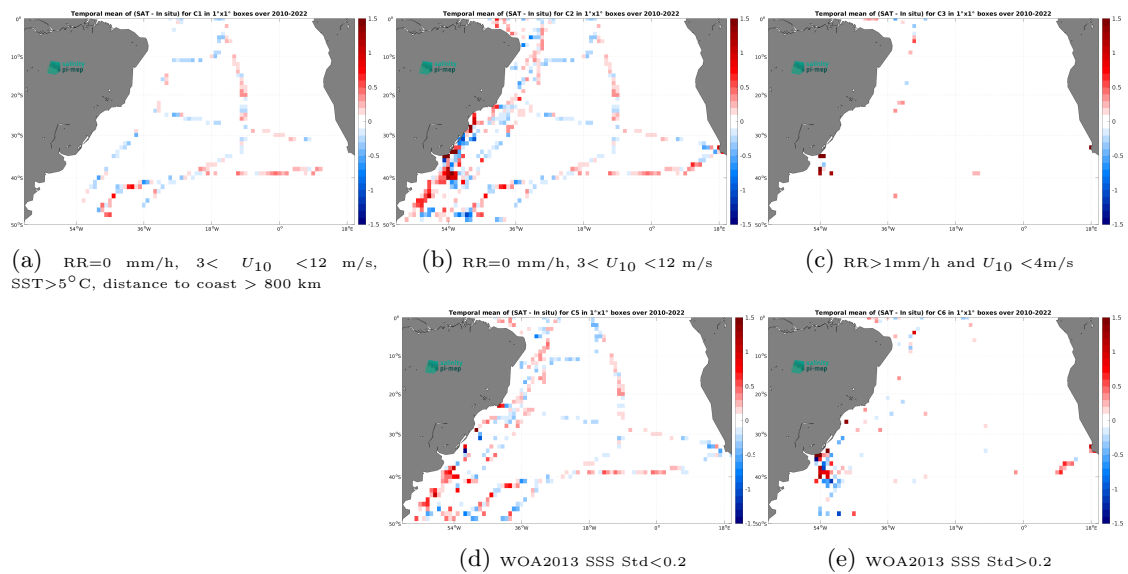
Figure 12: Temporal mean gridded over spatial boxes of size 1^\circ \times 1^\circ of \Delta\text{SSS} (SMOS SSS L3 v335 - 10 Days - 25 km (CATDS-CPDC) - TSG (CSIC-UTM)) for 5 different subdatasets corresponding to:RR=0 mm/h, 3 < U_{10} < 12 m/s, SST >5^\circ\text{C} , distance to coast > 800 km (a), RR=0 mm/h, 3 < U_{10} < 12 m/s (b), RR >1 mm/h and U_{10} < 4 m/s (c), WOA2013 SSS Std <0.2 (d), WOA2013 SSS Std >0.2 (e).
