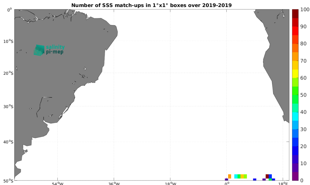
Figure 5: Number of SSS match-ups between Saildrone SSS and the SMOS SSS L3 v335 - 10 Days - 25 km (CATDS-CPDC) SSS product for the South Atlantic Ocean Pi-MEP region over 1^\circ \times 1^\circ boxes and for the full satellite product period.
