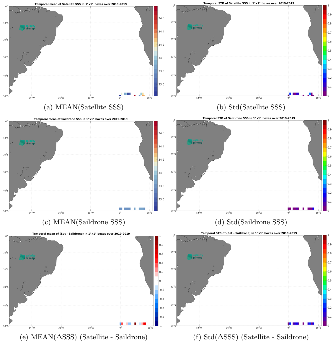
Figure 7: Temporal mean (left) and Std (right) of SSS from SMOS SSS L3 v335 - 10 Days - 25 km (CATDS-CPDC) (top), Saildrone (middle), and of \Delta SSS (Satellite - Saildrone). Only match-up pairs are used to generate these maps.
