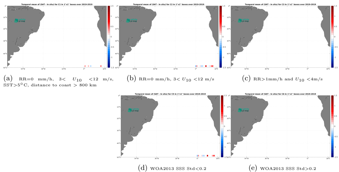
Figure 14: Temporal mean gridded over spatial boxes of size 1^\circ \times 1^\circ of \Delta SSS (SMOS SSS L3 v335 - 10 Days - 25 km (CATDS-CPDC) - Saildrone) for 5 different subdatasets corresponding to:RR=0 mm/h, 3 < U_{10} < 12 m/s, SST >5^\circ\text{C} , distance to coast > 800 km (a), RR=0 mm/h, 3 < U_{10} < 12 m/s (b), RR >1 mm/h and U_{10} < 4 m/s (c), WOA2013 SSS Std <0.2 (d), WOA2013 SSS Std >0.2 (e).
