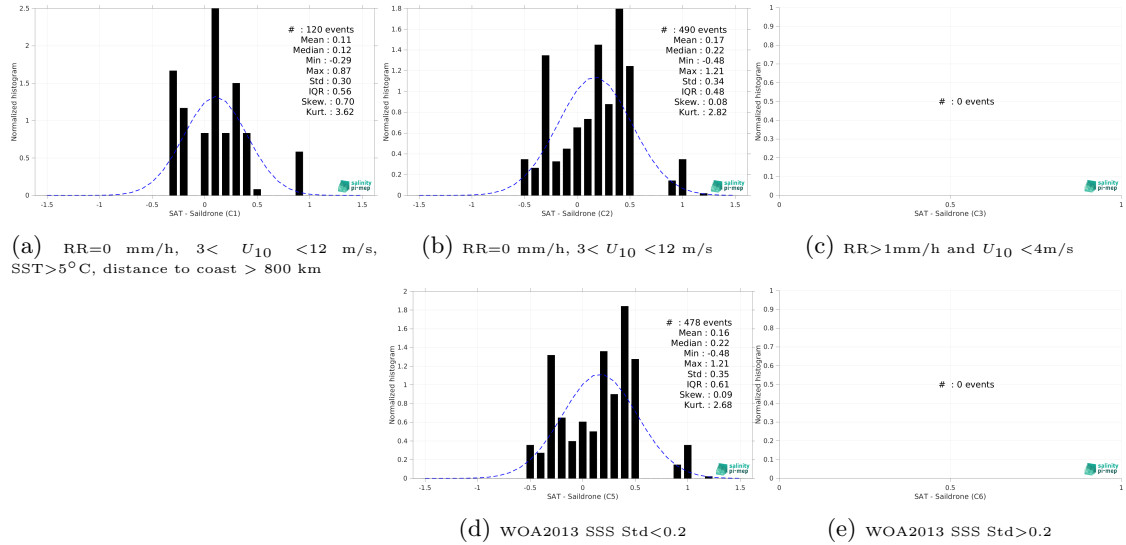
Figure 15: Normalized histogram of \Delta SSS (SMOS SSS L3 v335 - 10 Days - 25 km (CATDS-CPDC) - Saildrone) for 5 different subdatasets corresponding to: RR=0 mm/h, 3 < U_{10} < 12 m/s, SST > 5°C, distance to coast > 800 km (a), RR=0 mm/h, 3 < U_{10} < 12 m/s (b), RR > 1mm/h and U_{10} < 4 m/s (c), WOA2013 SSS Std < 0.2 (d), WOA2013 SSS Std > 0.2 (e).
