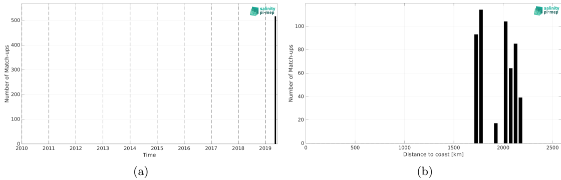
Figure 1: Number of match-ups between Saildrone and SMOS SSS L3 v335 - 10 Days - 25 km (CATDS-CPDC) SSS as a function of time (a) and as function of the distance to coast (b) over the South Atlantic Ocean Pi-MEP region and for the full satellite product period.
