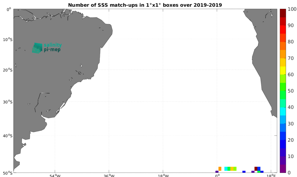
Figure 4: Number of SSS match-ups between Saildrone SSS and the SMOS SSS L3 v335 - 10 Days - 25 km (CATDS-CPDC) SSS product for the South Atlantic Ocean Pi-MEP region over 1^\circ \times 1^\circ boxes and for the full satellite product period.
