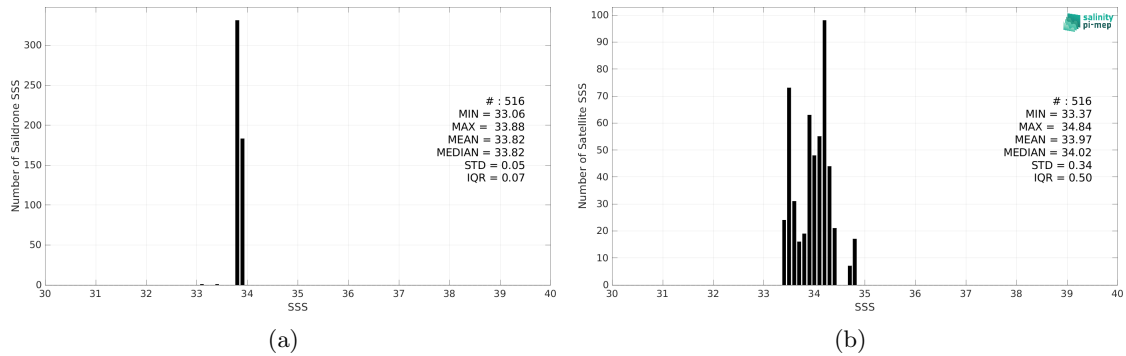
Figure 2: Histograms of SSS from Saildrone (a) and SMOS SSS L3 v335 - 10 Days - 25 km (CATDS-CPDC) (b) considering all match-up pairs per bins of 0.1 over the South Atlantic Ocean Pi-MEP region and for the full satellite product period.
