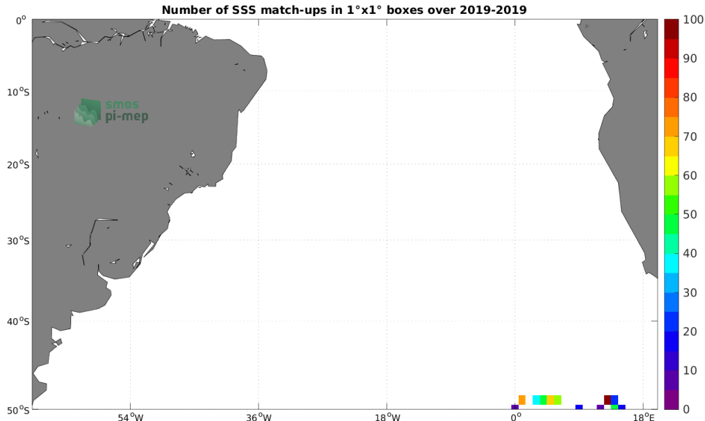
Figure 4: Number of SSS match-ups between Saildrone SSS and the SMOS SSS L3 v335 - 10 Days - 25 km (CATDS-CPDC) SSS product for the South Atlantic Ocean Pi-MEP region over 1^{\circ} \times 1^{\circ} boxes and for the full satellite product period.
