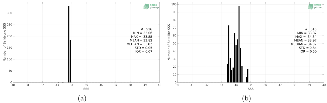
Figure 2: Histograms of SSS from Sairdrone (a) and SMOS SSS L3 v335 - 10 Days - 25 km (CATDS-CPDC) (b) considering all match-up pairs per bins of 0.1 over the South Atlantic Ocean Pi-MEP region and for the full satellite product period.
