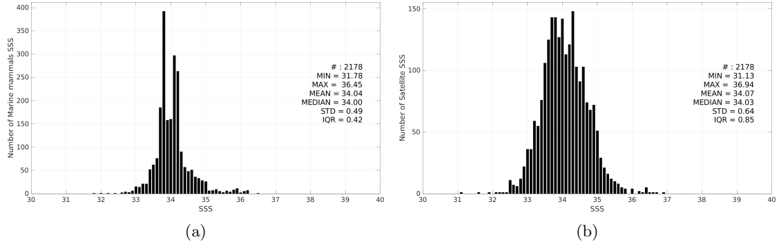
Figure 3: Histograms of SSS from Marine mammals (a) and SMOS SSS L3 v335 - 10 Days - 25 km (CATDS-CPDC) (b) considering all match-up pairs per bins of 0.1 over the South Atlantic Ocean Pi-MEP region and for the full satellite product period.
