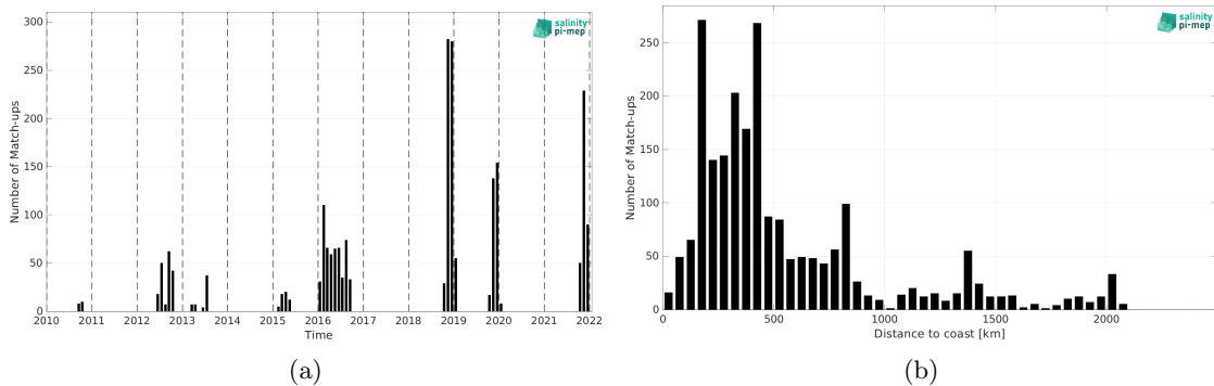
Figure 2: Number of match-ups between Marine mammals and SMOS SSS L3 v335 - 10 Days - 25 km (CATDS-CPDC) SSS as a function of time (a) and as function of the distance to coast (b) over the South Atlantic Ocean Pi-MEP region and for the full satellite product period.
