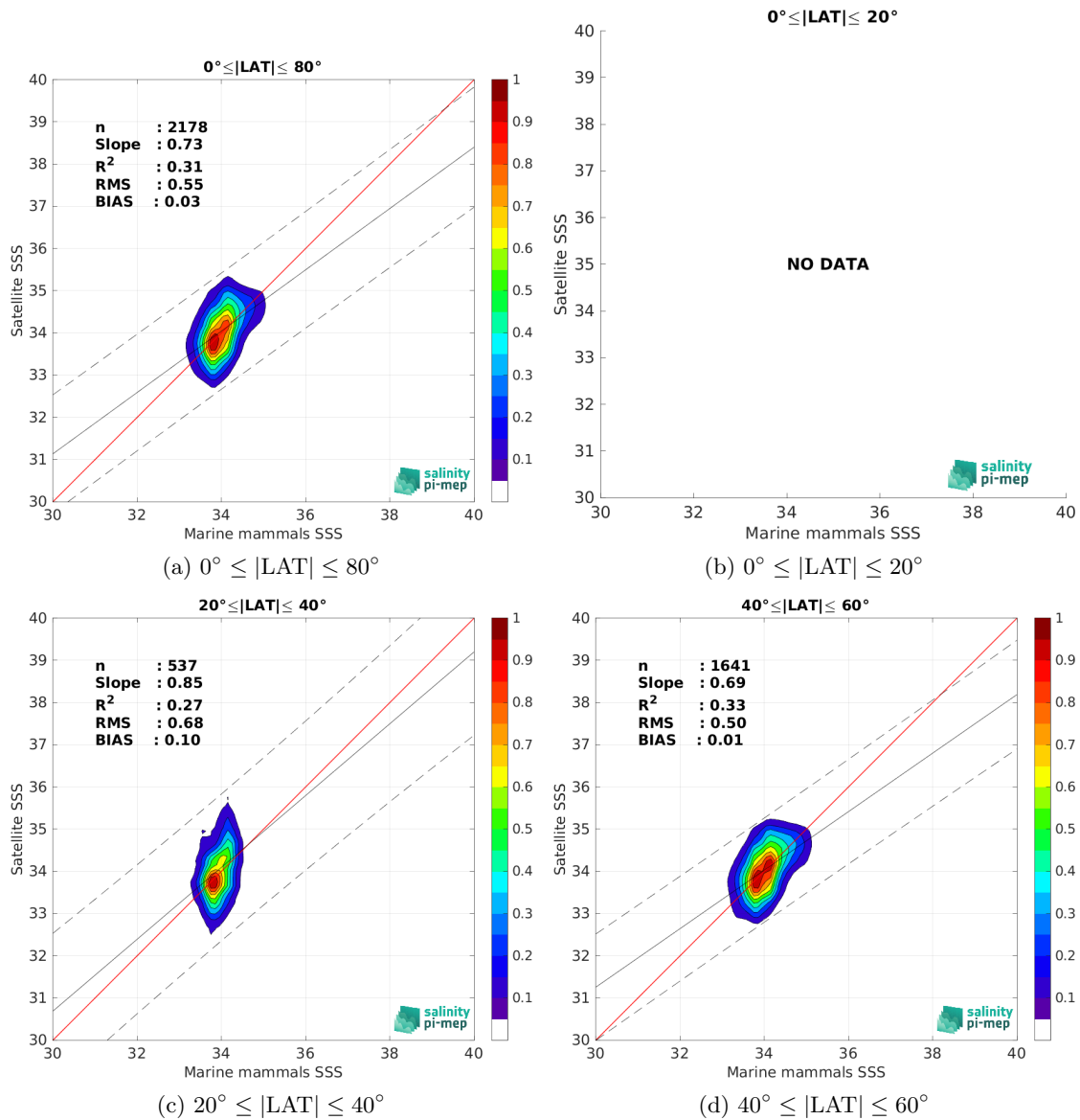
Figure 10: Contour maps of the concentration of SMOS SSS L3 v335 - 10 Days - 25 km (CATDS-CPDC) SSS (y-axis) versus Marine mammals SSS (x-axis) at match-up pairs for different latitude bands. For each plot, the red line shows x=y . The black thin and dashed lines indicate a linear fit through the data cloud and the \pm 95\% confidence levels, respectively. The number match-up pairs n , the slope and R^2 coefficient of the linear fit, the root mean square (RMS) and the mean bias between satellite and in situ data are indicated for each latitude band in each plots.
