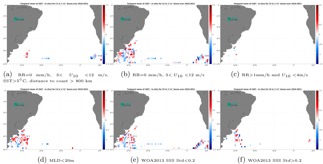
Figure 14: Temporal mean gridded over spatial boxes of size 1^\circ \times 1^\circ of \Delta SSS (SMOS SSS L3 v335 - 10 Days - 25 km (CATDS-CPDC) - Marine mammals) for 6 different subdatasets corresponding to:RR=0 mm/h, 3 < U_{10} < 12 m/s, SST>5°C, distance to coast > 800 km (a), RR=0 mm/h, 3 < U_{10} < 12 m/s (b), RR>1mm/h and U_{10} < 4 m/s (c),MLD<20m (d),WOA2013 SSS Std<0.2 (e),WOA2013 SSS Std>0.2 (f).
