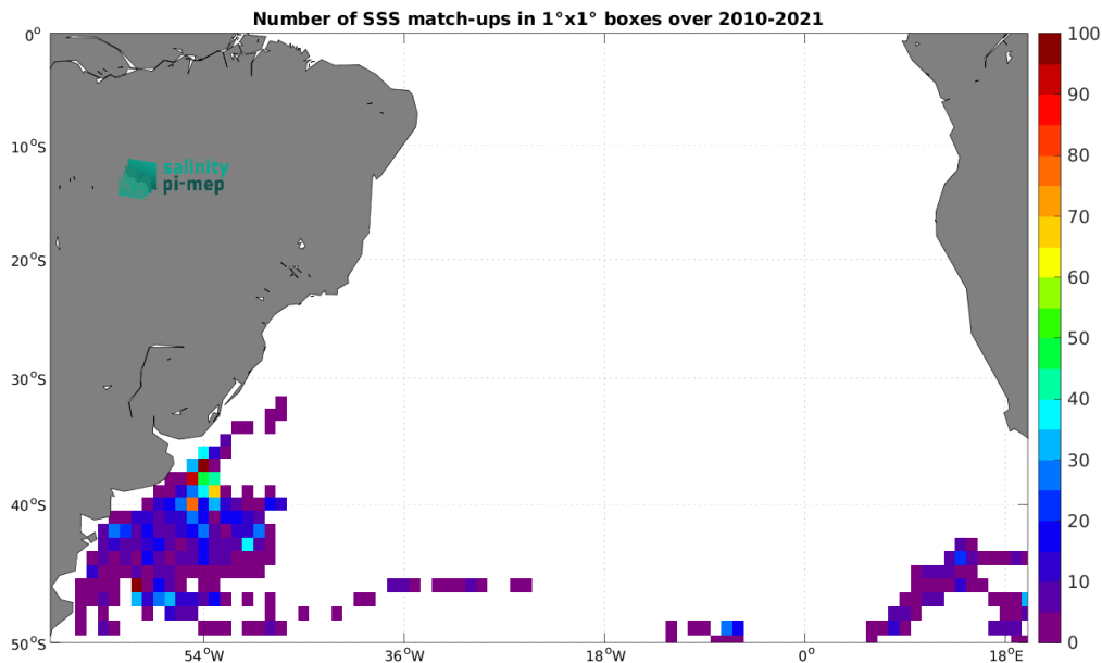
Figure 5: Number of SSS match-ups between Marine mammals SSS and the SMOS SSS L3 v335 - 10 Days - 25 km (CATDS-CPDC) SSS product for the South Atlantic Ocean Pi-MEP region over 1^\circ \times 1^\circ boxes and for the full satellite product period.
