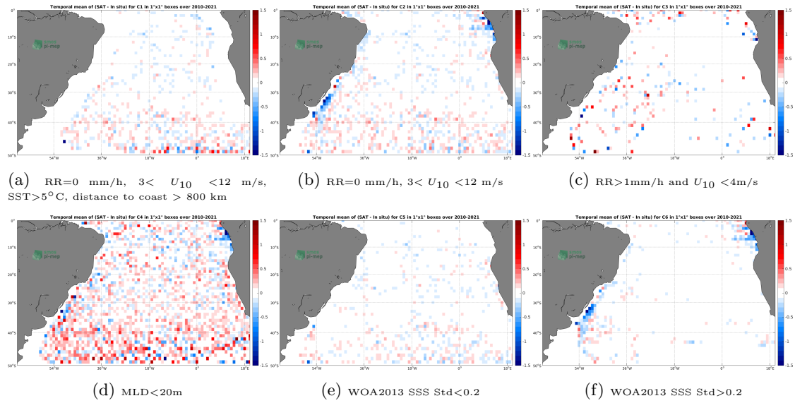
Figure 12: Temporal mean gridded over spatial boxes of size 1^\circ \times 1^\circ of \Delta SSS (SMOS SSS L3 v335 - 10 Days - 25 km (CATDS-CPDC) - Argo) for 6 different subdatasets corresponding to: RR=0 mm/h, 3 < U_{10} < 12 m/s, SST > 5^\circ C , distance to coast > 800 km (a), RR=0 mm/h, 3 < U_{10} < 12 m/s (b), RR > 1 mm/h and U_{10} < 4 m/s (c), MLD < 20 m (d), WOA2013 SSS Std < 0.2 (e), WOA2013 SSS Std > 0.2 (f).
