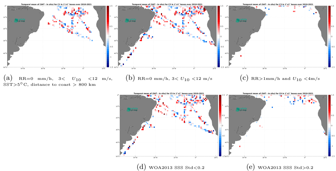
Figure 14: Temporal mean gridded over spatial boxes of size 1^\circ \times 1^\circ of \Delta\text{SSS} (SMOS SSS L2Q v333 - 0.25 Deg (CATDS-CPDC) - TSG (GOSUD-Research-vessel)) for 5 different subdatasets corresponding to:RR=0 mm/h, 3 < U_{10} < 12 m/s, SST>5°C, distance to coast > 800 km (a), RR=0 mm/h, 3 < U_{10} < 12 m/s (b), RR>1mm/h and U_{10} < 4 m/s (c), WOA2013 SSS Std<0.2 (d), WOA2013 SSS Std>0.2 (e).
