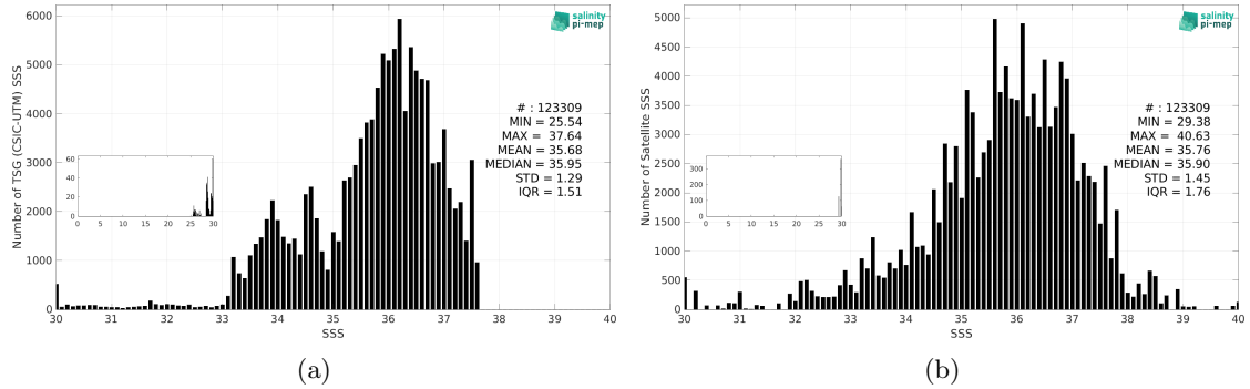
Figure 3: Histograms of SSS from TSG (CSIC-UTM) (a) and SMOS SSS L2Q v333 - 0.25 Deg (CATDS-CPDC) (b) considering all match-up pairs per bins of 0.1 over the South Atlantic Ocean Pi-MEP region and for the full satellite product period.
