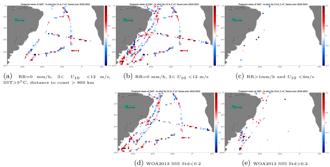
Figure 14: Temporal mean gridded over spatial boxes of size 1^\circ \times 1^\circ of \Delta\text{SSS} (SMOS SSS L2Q v333 - 0.25 Deg (CATDS-CPDC) - TSG (CSIC-UTM)) for 5 different subdatasets corresponding to:RR=0 mm/h, 3 < U_{10} < 12 m/s, SST >5^\circ\text{C} , distance to coast > 800 km (a), RR=0 mm/h, 3 < U_{10} < 12 m/s (b), RR >1 mm/h and U_{10} < 4 m/s (c), WOA2013 SSS Std <0.2 (d), WOA2013 SSS Std >0.2 (e).
