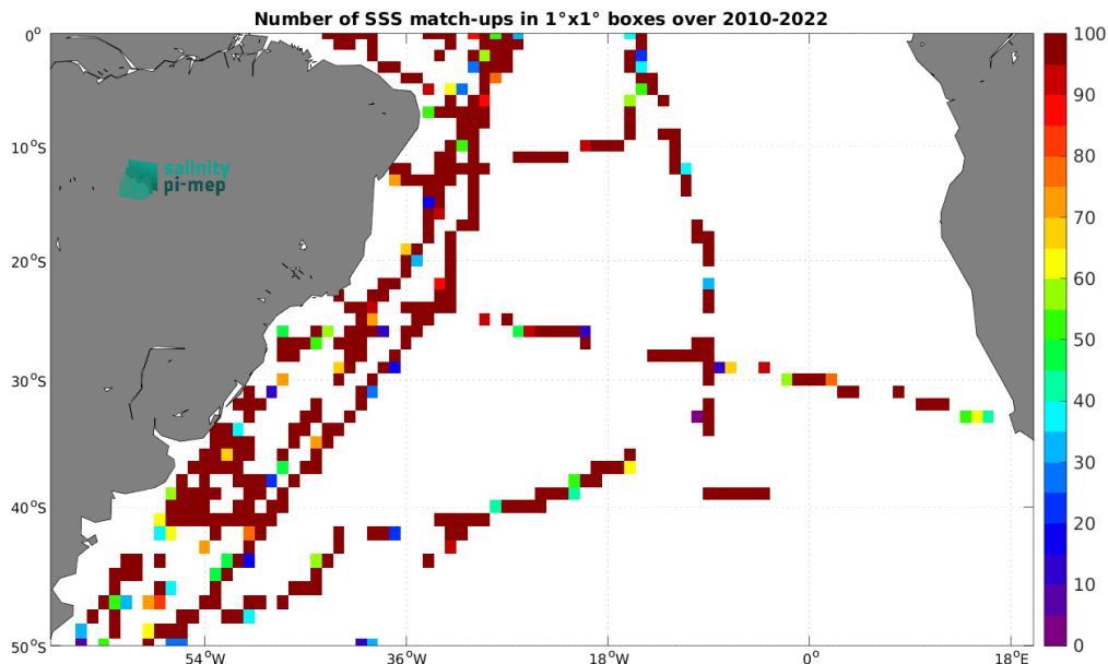
Figure 5: Number of SSS match-ups between TSG (CSIC-UTM) SSS and the SMOS SSS L2Q v333 - 0.25 Deg (CATDS-CPDC) SSS product for the South Atlantic Ocean Pi-MEP region over 1^\circ \times 1^\circ boxes and for the full satellite product period.
