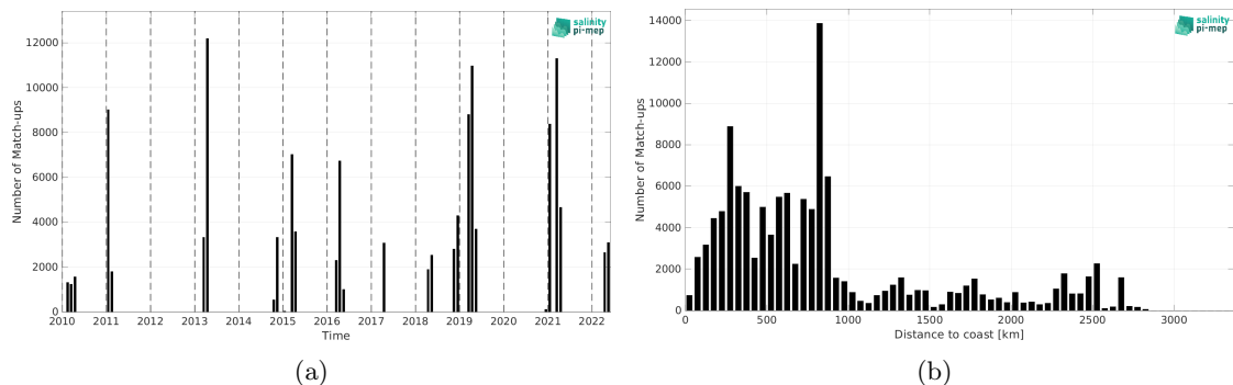
Figure 2: Number of match-ups between TSG (CSIC-UTM) and SMOS SSS L2Q v333 - 0.25 Deg (CATDS-CPDC) SSS as a function of time (a) and as function of the distance to coast (b) over the South Atlantic Ocean Pi-MEP region and for the full satellite product period.
