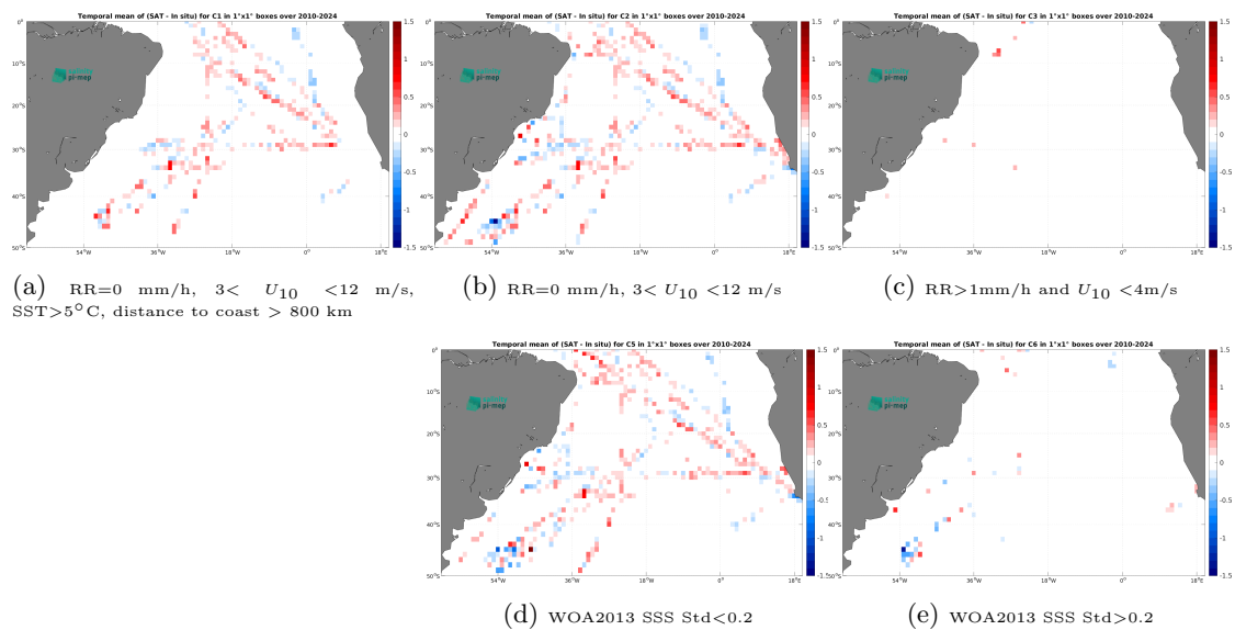
Figure 14: Temporal mean gridded over spatial boxes of size 1^\circ \times 1^\circ of \Delta SSS (SMOS SSS L3 v332 - 9 Days (CATDS-CPDC) - TSG (SAMOS)) for 5 different subdatasets corresponding to:RR=0 mm/h, 3 < U_{10} < 12 m/s, SST >5^\circ\text{C} , distance to coast > 800 km (a), RR=0 mm/h, 3 < U_{10} < 12 m/s (b), RR >1 mm/h and U_{10} < 4 m/s (c), WOA2013 SSS Std <0.2 (d), WOA2013 SSS Std >0.2 (e).
