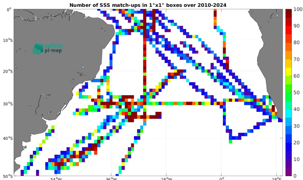
Figure 5: Number of SSS match-ups between TSG (SAMOS) SSS and the SMOS SSS L3 v332 - 9 Days (CATDS-CPDC) SSS product for the South Atlantic Ocean Pi-MEP region over 1^\circ \times 1^\circ boxes and for the full satellite product period.
