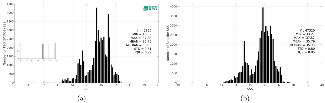
Figure 3: Histograms of SSS from TSG (SAMOS) (a) and SMOS SSS L3 v332 - 9 Days (CATDS-CPDC) (b) considering all match-up pairs per bins of 0.1 over the South Atlantic Ocean Pi-MEP region and for the full satellite product period.
