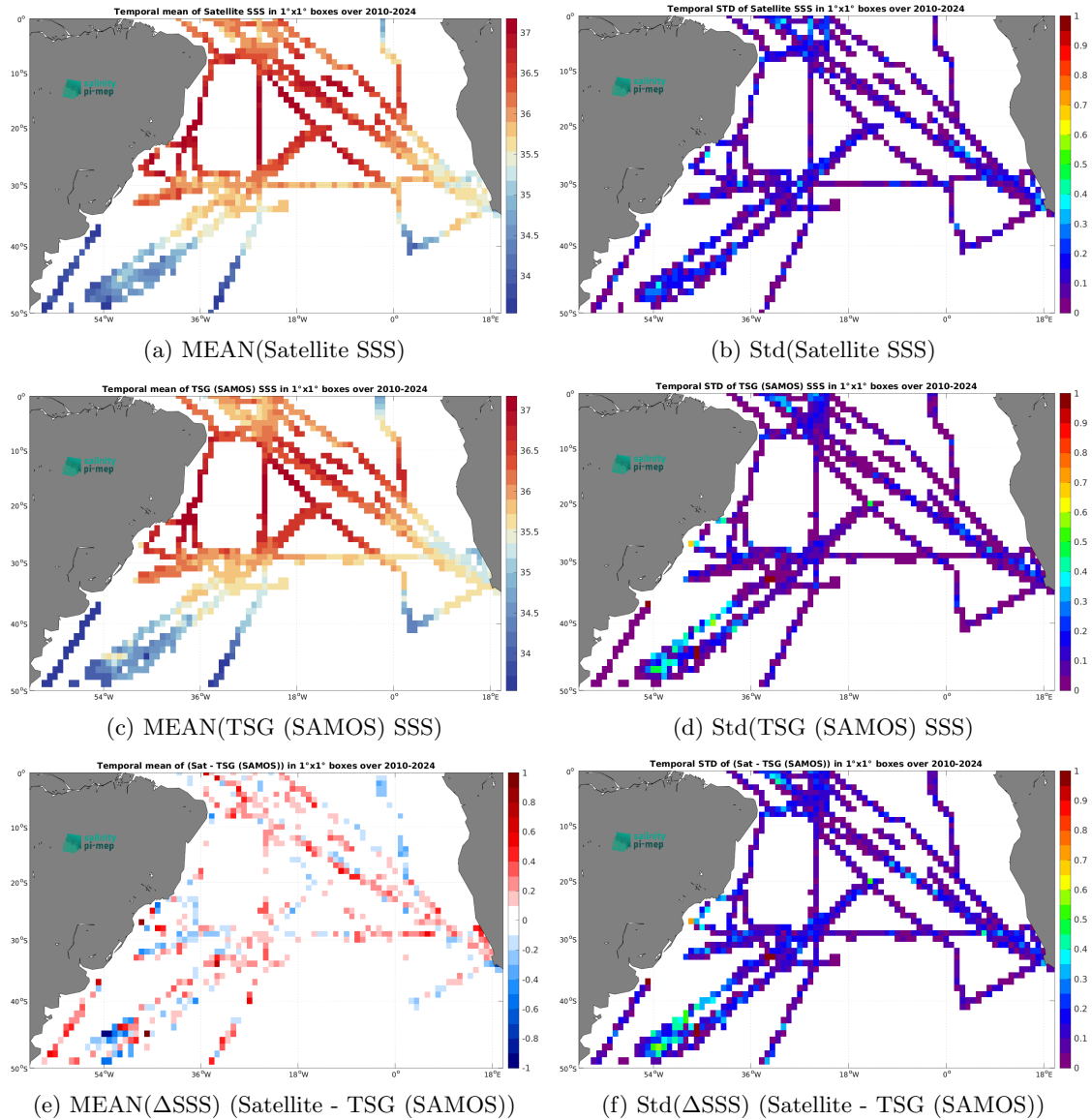
Figure 7: Temporal mean (left) and Std (right) of SSS from SMOS SSS L3 v332 - 9 Days (CATDS-CPDC) (top), TSG (SAMOS) (middle), and of \Delta SSS (Satellite - TSG (SAMOS)). Only match-up pairs are used to generate these maps.
