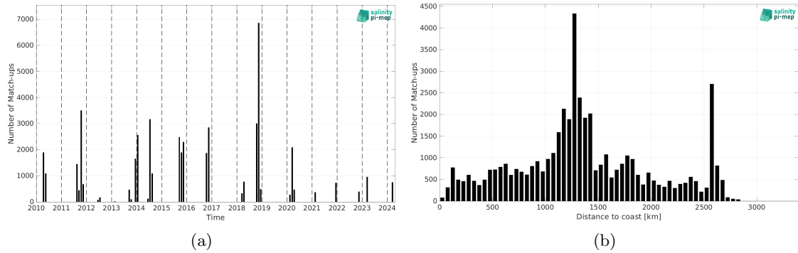
Figure 2: Number of match-ups between TSG (SAMOS) and SMOS SSS L3 v332 - 9 Days (CATDS-CPDC) SSS as a function of time (a) and as function of the distance to coast (b) over the South Atlantic Ocean Pi-MEP region and for the full satellite product period.
