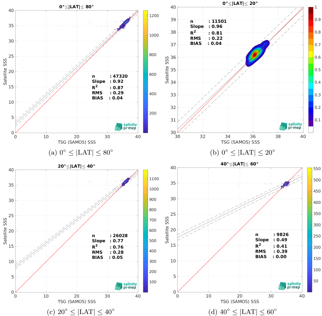
Figure 10: Contour maps of the concentration of SMOS SSS L3 v332 - 9 Days (CATDS-CPDC) SSS (y-axis) versus TSG (SAMOS) SSS (x-axis) at match-up pairs for different latitude bands. For each plot, the red line shows x=y . The black thin and dashed lines indicate a linear fit through the data cloud and the \pm 95\% confidence levels, respectively. The number match-up pairs n , the slope and R^2 coefficient of the linear fit, the root mean square (RMS) and the mean bias between satellite and in situ data are indicated for each latitude band in each plots.
