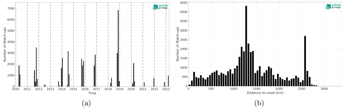
Figure 1: Number of match-ups between TSG (SAMOS) and SMOS SSS L3 v332 - 9 Days (CATDS-CPDC) SSS as a function of time (a) and as function of the distance to coast (b) over the South Atlantic Ocean Pi-MEP region and for the full satellite product period.
