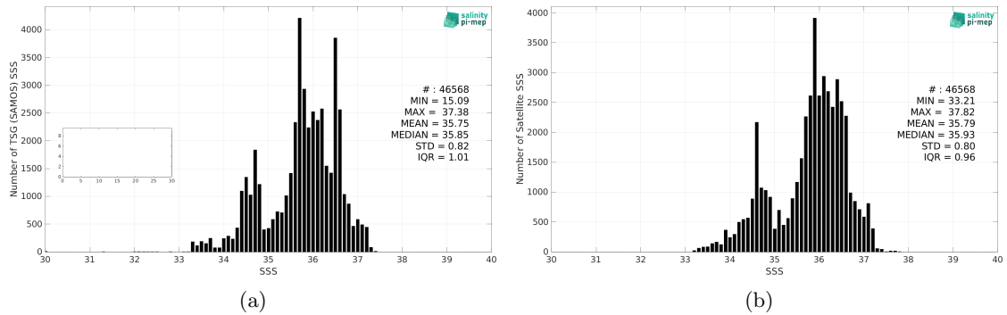
Figure 2: Histograms of SSS from TSG (SAMOS) (a) and SMOS SSS L3 v332 - 9 Days (CATDS-CPDC) (b) considering all match-up pairs per bins of 0.1 over the South Atlantic Ocean Pi-MEP region and for the full satellite product period.
