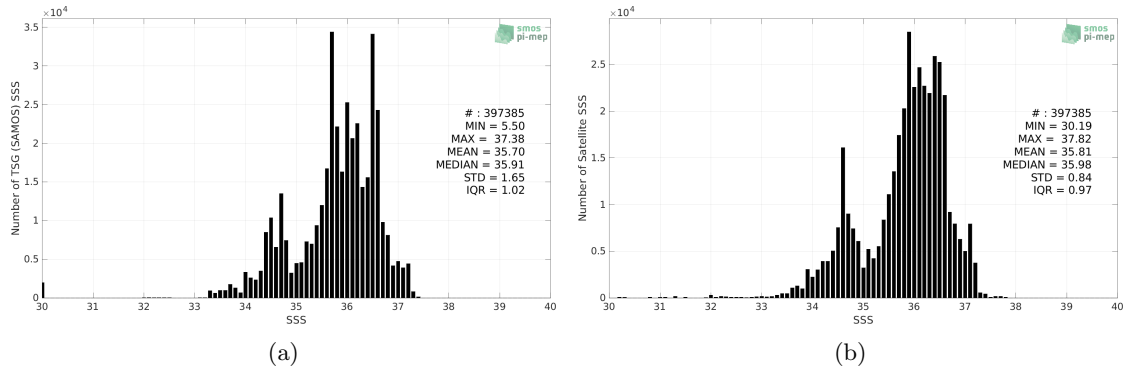
Figure 2: Histograms of SSS from TSG (SAMOS) (a) and SMOS SSS L3 v332 - 9 Days (CATDS-CPDC) (b) considering all match-up pairs per bins of 0.1 over the South Atlantic Ocean Pi-MEP region and for the full satellite product period.
