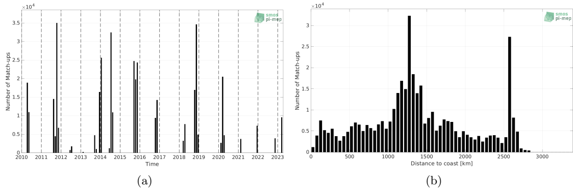
Figure 1: Number of match-ups between TSG (SAMOS) and SMOS SSS L3 v332 - 9 Days (CATDS-CPDC) SSS as a function of time (a) and as function of the distance to coast (b) over the South Atlantic Ocean Pi-MEP region and for the full satellite product period.
