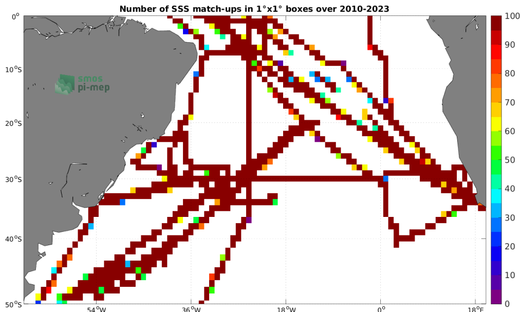
Figure 4: Number of SSS match-ups between TSG (SAMOS) SSS and the SMOS SSS L3 v332 - 9 Days (CATDS-CPDC) SSS product for the South Atlantic Ocean Pi-MEP region over 1^\circ \times 1^\circ boxes and for the full satellite product period.
