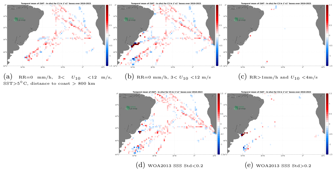
Figure 12: Temporal mean gridded over spatial boxes of size 1^\circ \times 1^\circ of \Delta\text{SSS} (SMOS SSS L3 v332 - 9 Days (CATDS-CPDC) - TSG (SAMOS)) for 5 different subdatasets corresponding to:RR=0 mm/h, 3 < U_{10} < 12 m/s, SST >5^\circ\text{C} , distance to coast > 800 km (a), RR=0 mm/h, 3 < U_{10} < 12 m/s (b), RR >1 mm/h and U_{10} < 4 m/s (c), WOA2013 SSS Std <0.2 (d), WOA2013 SSS Std >0.2 (e).
