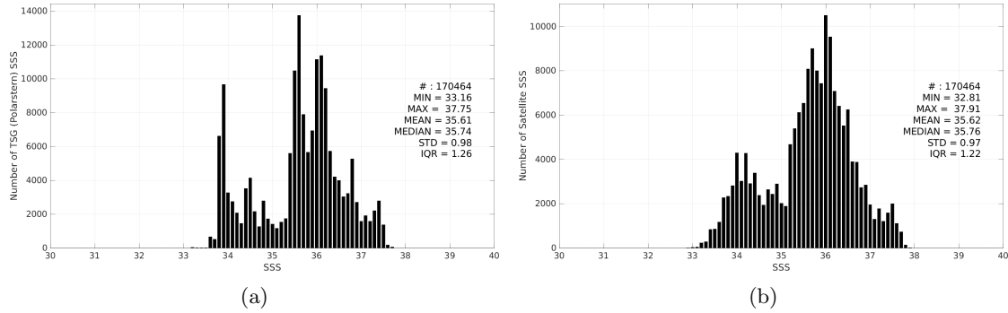
Figure 3: Histograms of SSS from TSG (Polarstern) (a) and SMOS SSS L3 v332 - 9 Days (CATDS-CPDC) (b) considering all match-up pairs per bins of 0.1 over the South Atlantic Ocean Pi-MEP region and for the full satellite product period.
