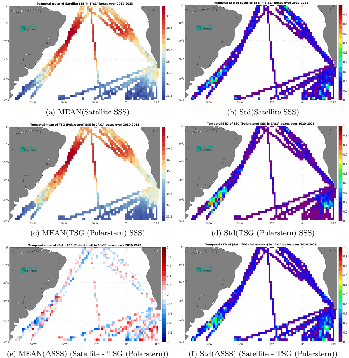
Figure 7: Temporal mean (left) and Std (right) of SSS from SMOS SSS L3 v332 - 9 Days (CATDS-CPDC) (top), TSG (Polarstern) (middle), and of \Delta SSS (Satellite - TSG (Polarstern)). Only match-up pairs are used to generate these maps.
