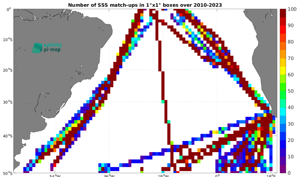
Figure 5: Number of SSS match-ups between TSG (Polarstern) SSS and the SMOS SSS L3 v332 - 9 Days (CATDS-CPDC) SSS product for the South Atlantic Ocean Pi-MEP region over 1^\circ \times 1^\circ boxes and for the full satellite product period.
