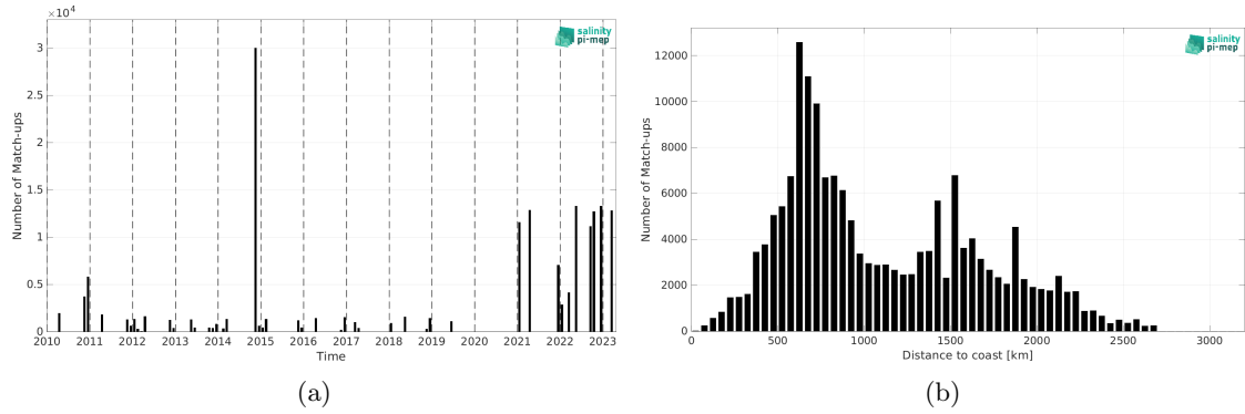
Figure 2: Number of match-ups between TSG (Polarstern) and SMOS SSS L3 v332 - 9 Days (CATDS-CPDC) SSS as a function of time (a) and as function of the distance to coast (b) over the South Atlantic Ocean Pi-MEP region and for the full satellite product period.
