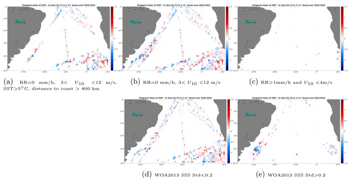
Figure 14: Temporal mean gridded over spatial boxes of size 1^\circ \times 1^\circ of \Delta SSS (SMOS SSS L3 v332 - 9 Days (CATDS-CPDC) - TSG (Polarstern)) for 5 different subdatasets corresponding to:RR=0 mm/h, 3 < U_{10} < 12 m/s, SST >5^\circ\text{C} , distance to coast > 800 km (a), RR=0 mm/h, 3 < U_{10} < 12 m/s (b), RR >1 mm/h and U_{10} < 4 m/s (c), WOA2013 SSS Std <0.2 (d), WOA2013 SSS Std >0.2 (e).
